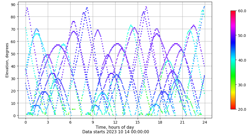
Time-elevation plot for station YEB1. Signal to Noise S1C Data file YEB100ESP_R_2023287.xtr
