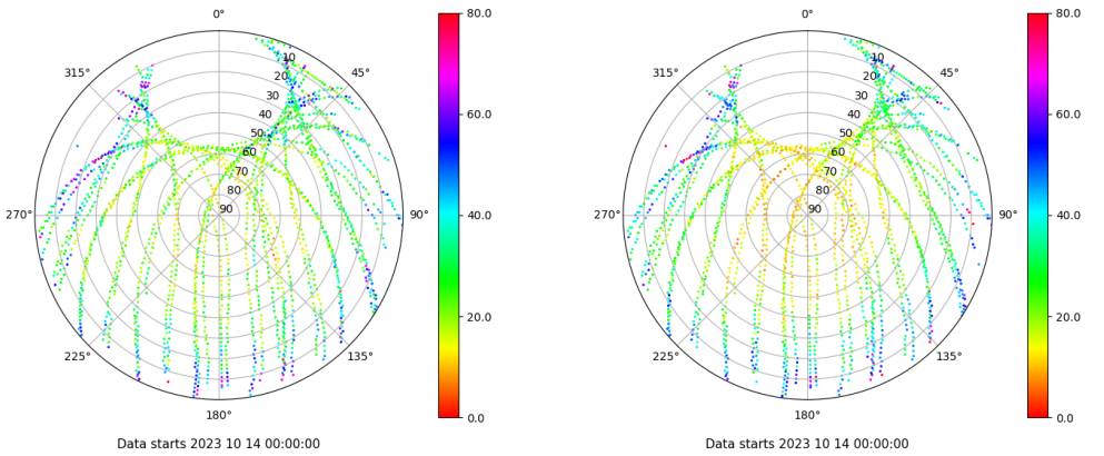
Skyplot for station YEB1. Parameter M1C Data file YEB100ESP_R_2023287.xtr Skyplot for station YEB1. Parameter M2P Data file YEB100ESP_R_2023287.xtr
