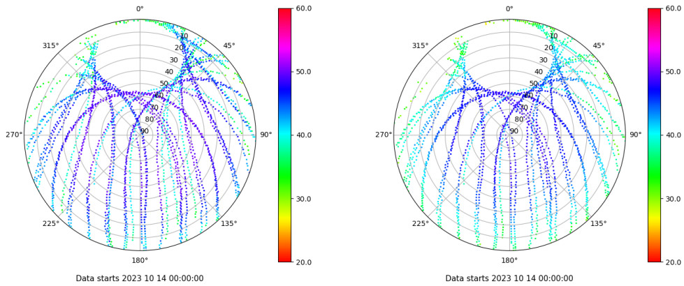
Skyplot for station YEB1. Signal to Noise S1C Data file YEB100ESP_R_2023287.xtr Skyplot for station YEB1. Signal to Noise S2P Data file YEB100ESP_R_2023287.xtr
