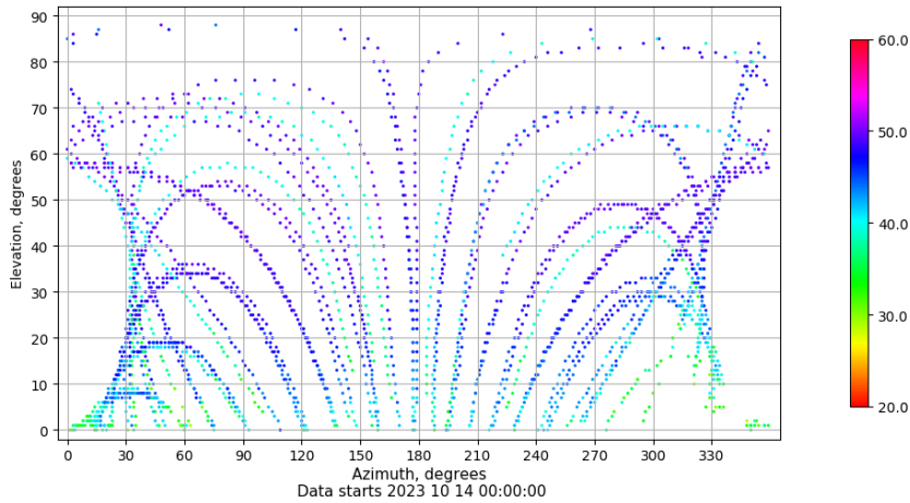
Azimuth-elevation plot for station YEB1. Signal to Noise S1C Data file YEB100ESP_R_2023287.xtr
