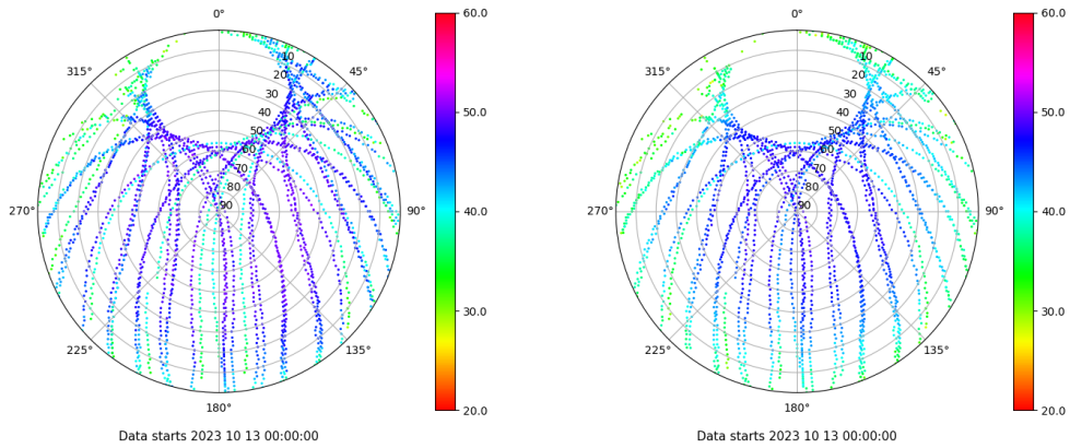
Skyplot for station YEB1. Signal to Noise S1C Data file YEB100ESP_R_2023286.xtr Skyplot for station YEB1. Signal to Noise S2P Data file YEB100ESP_R_2023286.xtr
