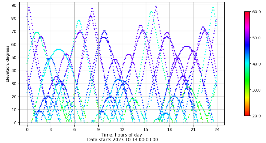
Time-elevation plot for station YEB1. Signal to Noise S1C Data file YEB100ESP_R_2023286.xtr
