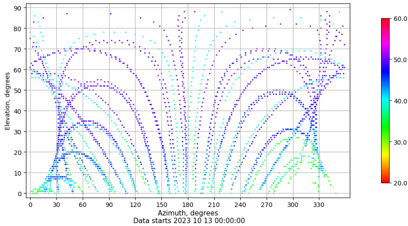
Azimuth-elevation plot for station YEB1. Signal to Noise S1C Data file YEB100ESP_R_2023286.xtr
