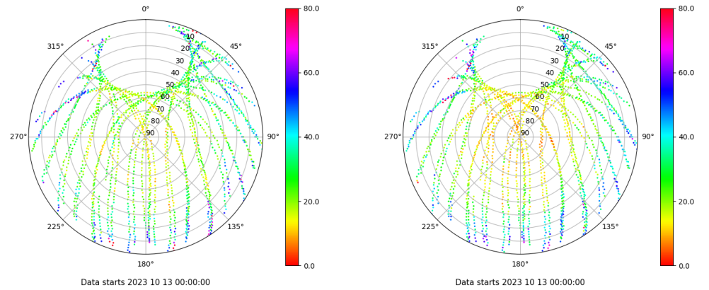
Skyplot for station YEB1. Parameter M1C Data file YEB100ESP_R_2023286.xtr Skyplot for station YEB1. Parameter M2P Data file YEB100ESP_R_2023286.xtr
