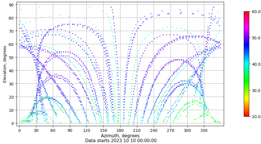
Azimuth-elevation plot for station YEB1. Signal to Noise S1C Data file YEB100ESP_R_2023283.xtr
