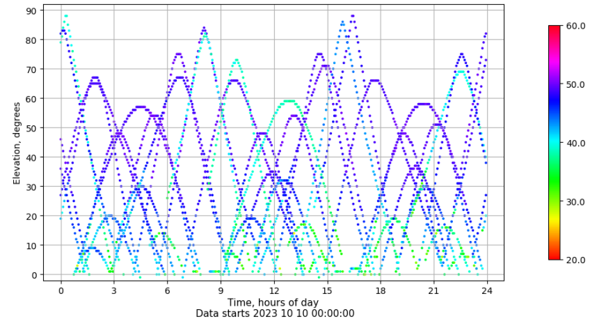
Time-elevation plot for station YEB1. Signal to Noise S1C Data file YEB100ESP_R_2023283.xtr
