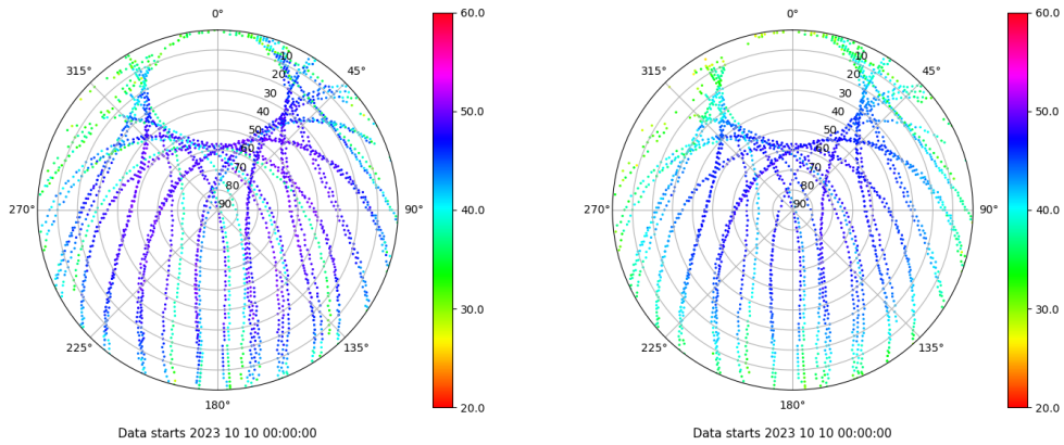
Skyplot for station YEB1. Signal to Noise S1C Data file YEB100ESP_R_2023283.xtr Skyplot for station YEB1. Signal to Noise S2P Data file YEB100ESP_R_2023283.xtr
