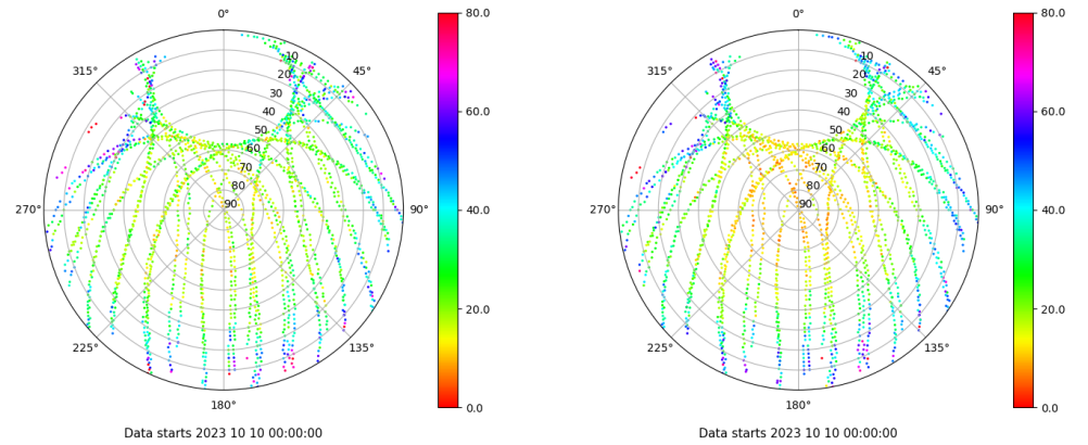
Skyplot for station YEB1. Parameter M1C Data file YEB100ESP_R_2023283.xtr Skyplot for station YEB1. Parameter M2P Data file YEB100ESP_R_2023283.xtr
