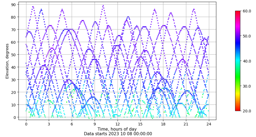
Time-elevation plot for station YEB1. Signal to Noise S1C Data file YEB100ESP_R_2023281.xtr
