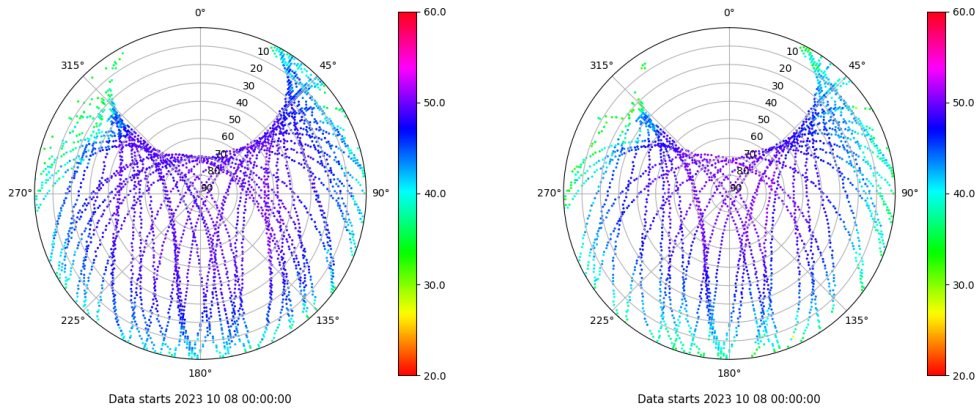
Skyplot for station YEB1. Signal to Noise S1C Data file YEB100ESP_R_2023281.xtr Skyplot for station YEB1. Signal to Noise S2S Data file YEB100ESP_R_2023281.xtr
