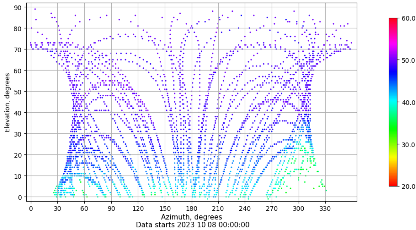
Azimuth-elevation plot for station YEB1. Signal to Noise S1C Data file YEB100ESP_R_2023281.xtr
