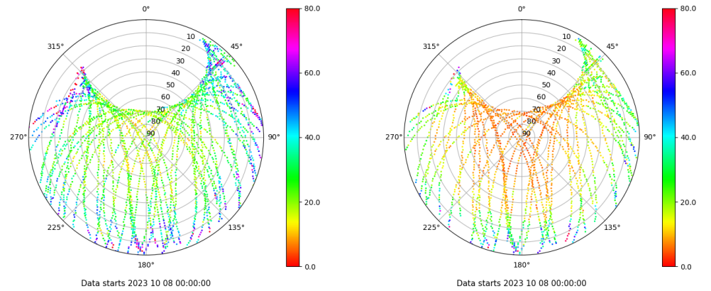
Skyplot for station YEB1. Parameter M1C Data file YEB100ESP_R_2023281.xtr Skyplot for station YEB1. Parameter M2S Data file YEB100ESP_R_2023281.xtr
