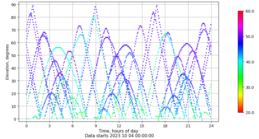
Time-elevation plot for station YEB1. Signal to Noise S1C Data file YEB100ESP_R_2023277.xtr
