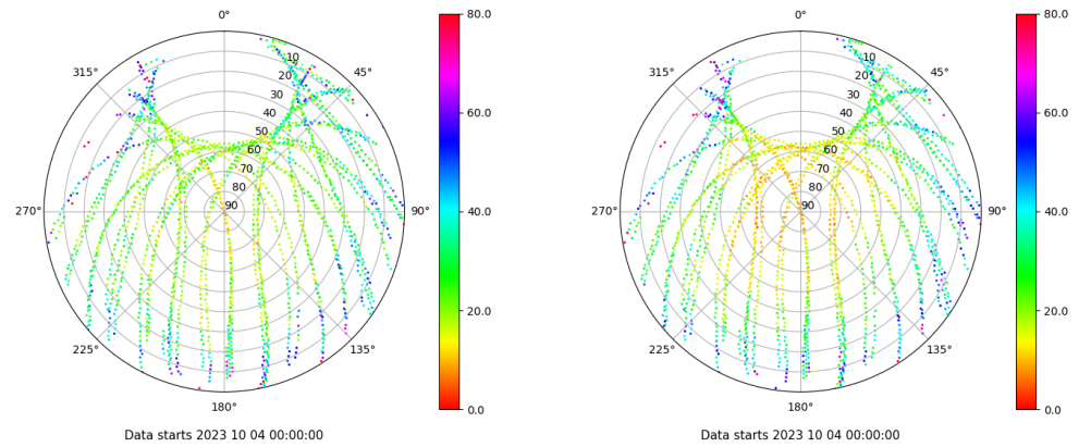
Skyplot for station YEB1. Parameter M1C Data file YEB100ESP_R_2023277.xtr Skyplot for station YEB1. Parameter M2P Data file YEB100ESP_R_2023277.xtr
