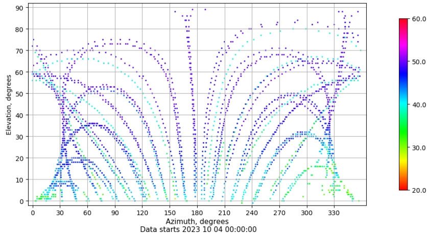
Azimuth-elevation plot for station YEB1. Signal to Noise S1C Data file YEB100ESP_R_2023277.xtr
