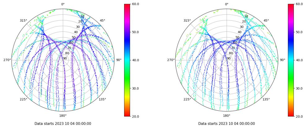
Skyplot for station YEB1. Signal to Noise S1C Data file YEB100ESP_R_2023277.xtr Skyplot for station YEB1. Signal to Noise S2P Data file YEB100ESP_R_2023277.xtr
