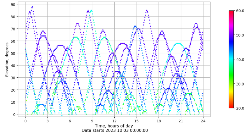
Time-elevation plot for station YEB1. Signal to Noise S1C Data file YEB100ESP_R_2023276.xtr
