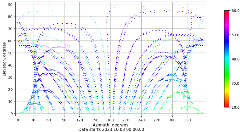
Azimuth-elevation plot for station YEB1. Signal to Noise S1C Data file YEB100ESP_R_2023276.xtr
