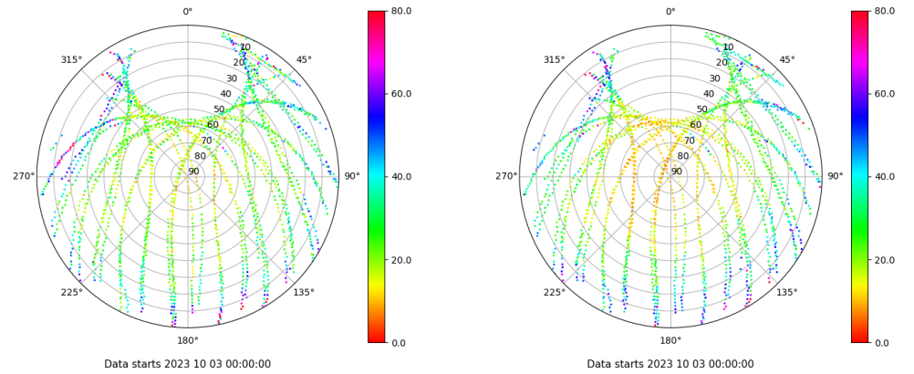
Skyplot for station YEB1. Parameter M1C Data file YEB100ESP_R_2023276.xtr Skyplot for station YEB1. Parameter M2P Data file YEB100ESP_R_2023276.xtr
