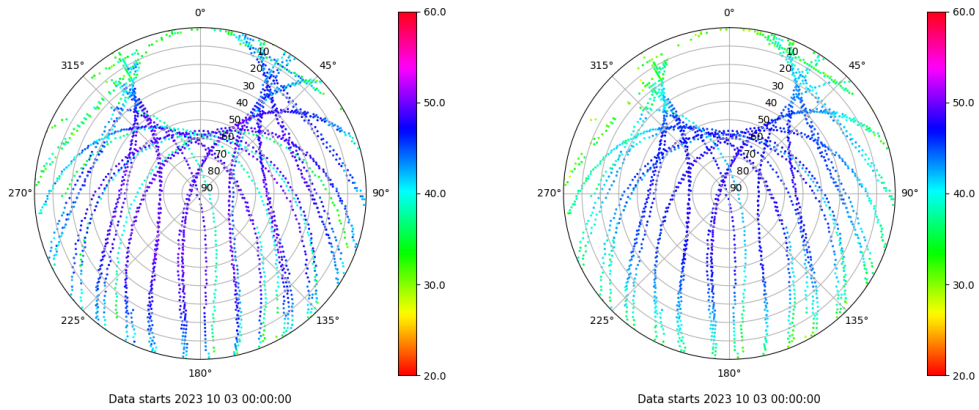
Skyplot for station YEB1. Signal to Noise S1C Data file YEB100ESP_R_2023276.xtr Skyplot for station YEB1. Signal to Noise S2P Data file YEB100ESP_R_2023276.xtr
