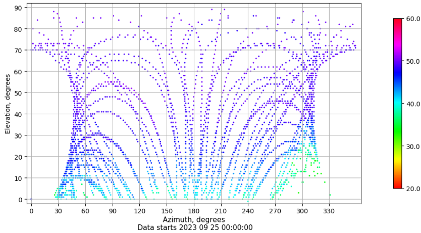
Azimuth-elevation plot for station YEB1. Signal to Noise S1C Data file YEB100ESP_R_2023268.xtr
