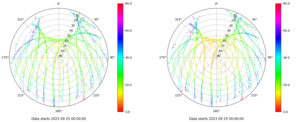
Skyplot for station YEB1. Parameter M1C Data file YEB100ESP_R_2023268.xtr Skyplot for station YEB1. Parameter M2P Data file YEB100ESP_R_2023268.xtr
