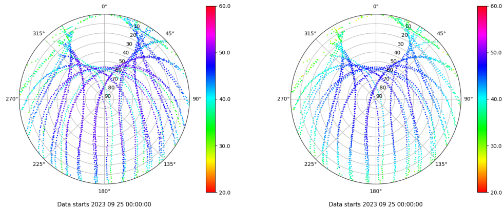
Skyplot for station YEB1. Signal to Noise S1C Data file YEB100ESP_R_2023268.xtr Skyplot for station YEB1. Signal to Noise S2P Data file YEB100ESP_R_2023268.xtr
