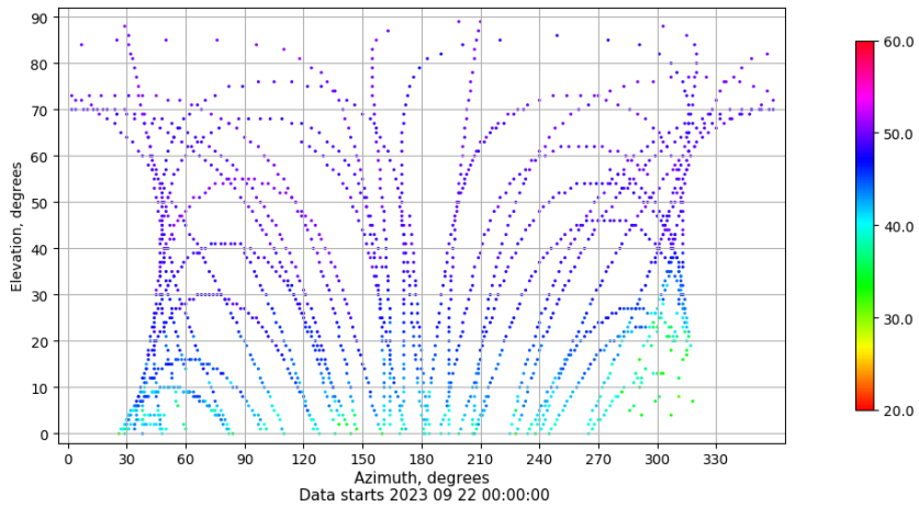
Azimuth-elevation plot for station YEB1. Signal to Noise S1C Data file YEB100ESP_R_2023265.xtr
