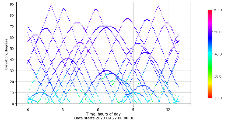
Time-elevation plot for station YEB1. Signal to Noise S1C Data file YEB100ESP_R_2023265.xtr
