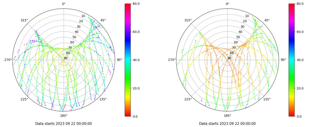
Skyplot for station YEB1. Parameter M1C Data file YEB100ESP_R_2023265.xtr Skyplot for station YEB1. Parameter M2S Data file YEB100ESP_R_2023265.xtr
