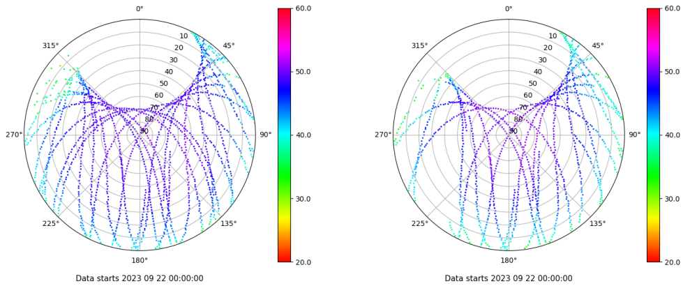
Skyplot for station YEB1. Signal to Noise S1C Data file YEB100ESP_R_2023265.xtr Skyplot for station YEB1. Signal to Noise S2S Data file YEB100ESP_R_2023265.xtr
