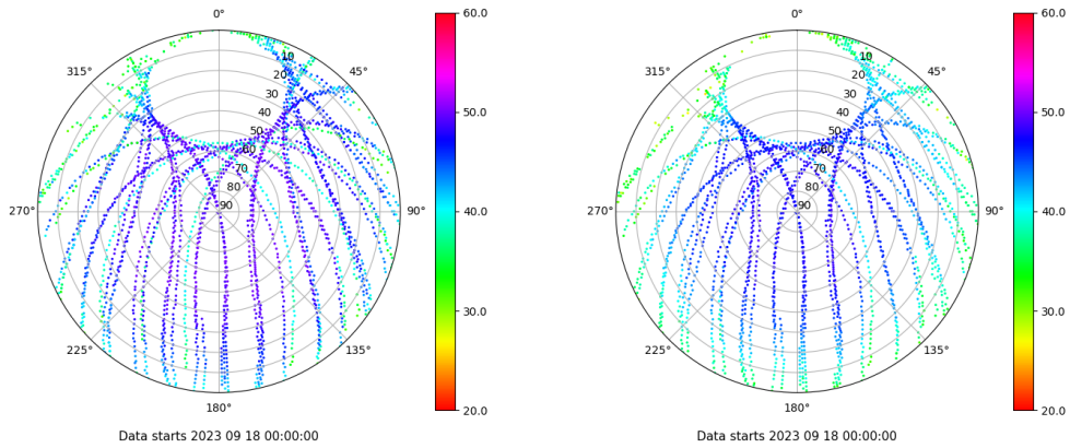
Skyplot for station YEB1. Signal to Noise S1C Data file YEB100ESP_R_2023261.xtr Skyplot for station YEB1. Signal to Noise S2P Data file YEB100ESP_R_2023261.xtr
