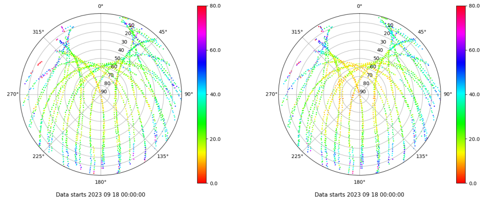
Skyplot for station YEB1. Parameter M1C Data file YEB100ESP_R_2023261.xtr Skyplot for station YEB1. Parameter M2P Data file YEB100ESP_R_2023261.xtr
