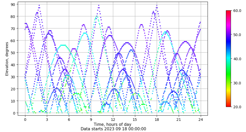
Time-elevation plot for station YEB1. Signal to Noise S1C Data file YEB100ESP_R_2023261.xtr
