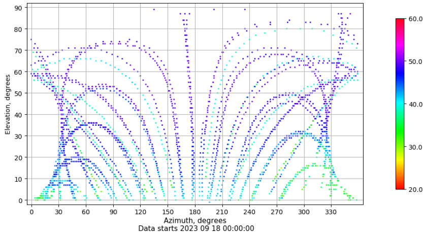
Azimuth-elevation plot for station YEB1. Signal to Noise S1C Data file YEB100ESP_R_2023261.xtr
