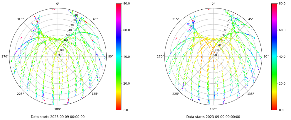
Skyplot for station YEB1. Parameter M1C Data file YEB100ESP_R_2023252.xtr Skyplot for station YEB1. Parameter M2P Data file YEB100ESP_R_2023252.xtr
