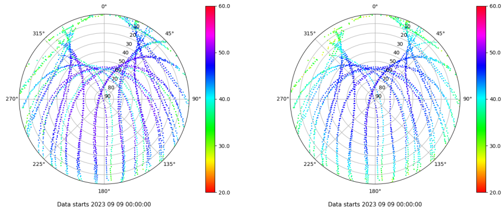
Skyplot for station YEB1. Signal to Noise S1C Data file YEB100ESP_R_2023252.xtr Skyplot for station YEB1. Signal to Noise S2P Data file YEB100ESP_R_2023252.xtr
