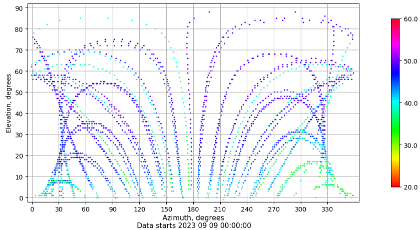
Azimuth-elevation plot for station YEB1. Signal to Noise S1C Data file YEB100ESP_R_2023252.xtr
