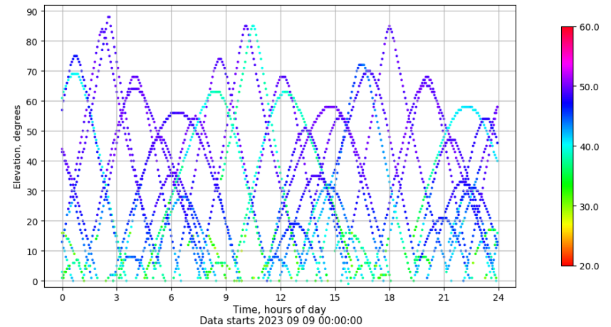
Time-elevation plot for station YEB1. Signal to Noise S1C Data file YEB100ESP_R_2023252.xtr
