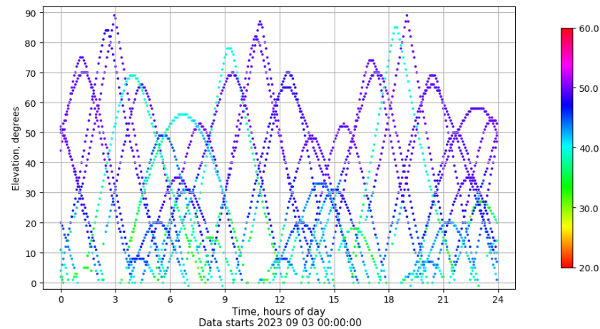
Time-elevation plot for station YEB1. Signal to Noise S1C Data file YEB100ESP_R_2023246.xtr
