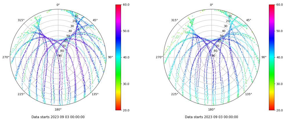
Skyplot for station YEB1. Signal to Noise S1C Data file YEB100ESP_R_2023246.xtr Skyplot for station YEB1. Signal to Noise S2P Data file YEB100ESP_R_2023246.xtr
