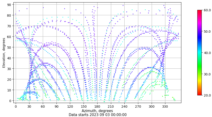
Azimuth-elevation plot for station YEB1. Signal to Noise S1C Data file YEB100ESP_R_2023246.xtr
