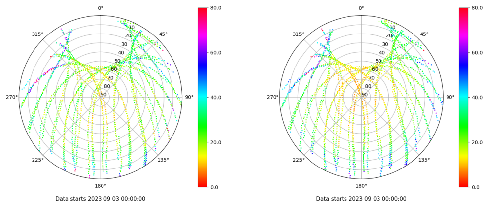
Skyplot for station YEB1. Parameter M1C Data file YEB100ESP_R_2023246.xtr Skyplot for station YEB1. Parameter M2P Data file YEB100ESP_R_2023246.xtr
