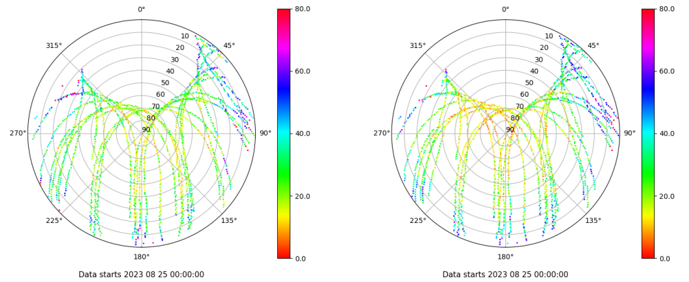
Skyplot for station YEB1. Parameter M1C Data file YEB100ESP_R_2023237.xtr Skyplot for station YEB1. Parameter M5Q Data file YEB100ESP_R_2023237.xtr
