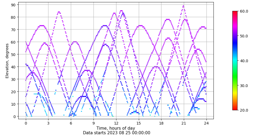
Time-elevation plot for station YEB1. Signal to Noise S1C Data file YEB100ESP_R_2023237.xtr
