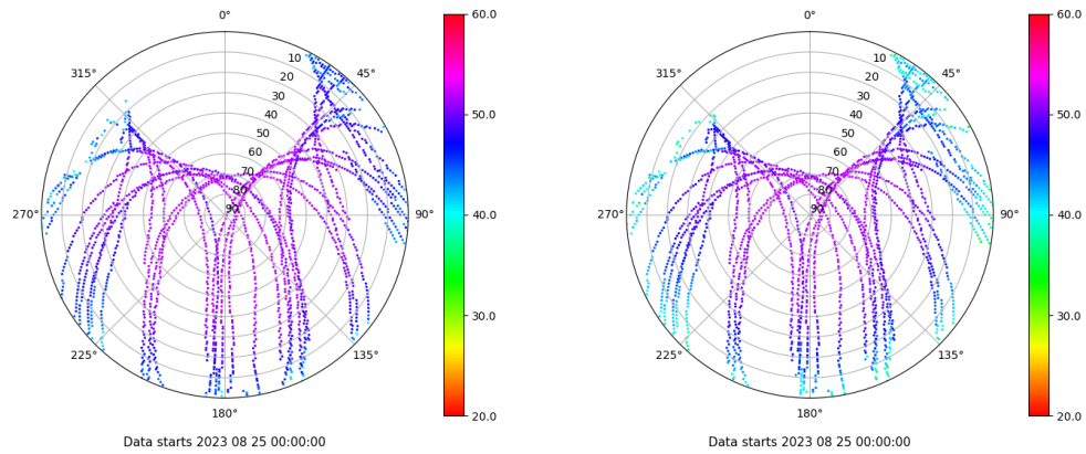
Skyplot for station YEB1. Signal to Noise S1C Data file YEB100ESP_R_2023237.xtr Skyplot for station YEB1. Signal to Noise S5Q Data file YEB100ESP_R_2023237.xtr
