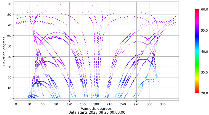
Azimuth-elevation plot for station YEB1. Signal to Noise S1C Data file YEB100ESP_R_2023237.xtr
