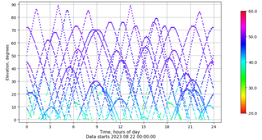
Time-elevation plot for station YEB1. Signal to Noise S1C Data file YEB100ESP_R_2023234.xtr
