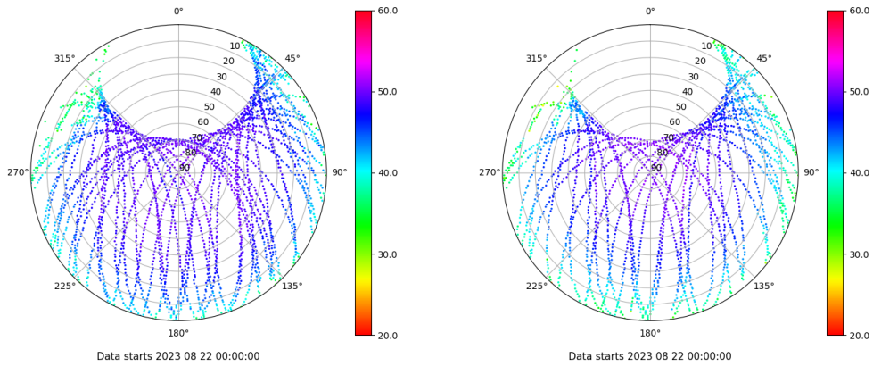
Skyplot for station YEB1. Signal to Noise S1C Data file YEB100ESP_R_2023234.xtr Skyplot for station YEB1. Signal to Noise S2S Data file YEB100ESP_R_2023234.xtr
