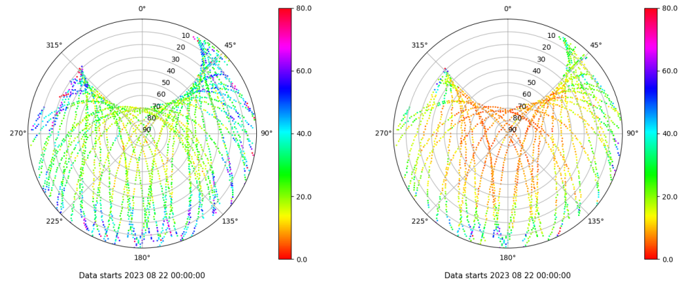
Skyplot for station YEB1. Parameter M1C Data file YEB100ESP_R_2023234.xtr Skyplot for station YEB1. Parameter M2S Data file YEB100ESP_R_2023234.xtr
