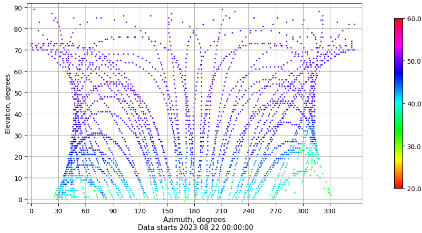
Azimuth-elevation plot for station YEB1. Signal to Noise S1C Data file YEB100ESP_R_2023234.xtr
