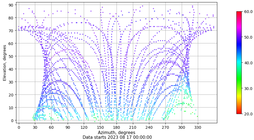
Azimuth-elevation plot for station YEB1. Signal to Noise S1C Data file YEB100ESP_R_2023229.xtr
