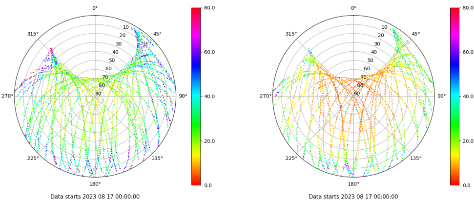
Skyplot for station YEB1. Parameter M1C Data file YEB100ESP_R_2023229.xtr Skyplot for station YEB1. Parameter M2S Data file YEB100ESP_R_2023229.xtr
