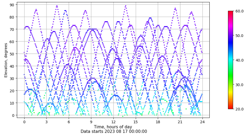
Time-elevation plot for station YEB1. Signal to Noise S1C Data file YEB100ESP_R_2023229.xtr
