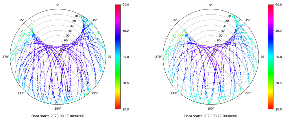
Skyplot for station YEB1. Signal to Noise S1C Data file YEB100ESP_R_2023229.xtr Skyplot for station YEB1. Signal to Noise S2S Data file YEB100ESP_R_2023229.xtr
