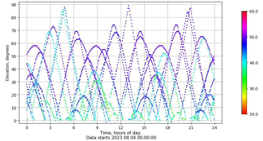
Time-elevation plot for station YEB1. Signal to Noise S1C Data file YEB100ESP_R_2023216.xtr
