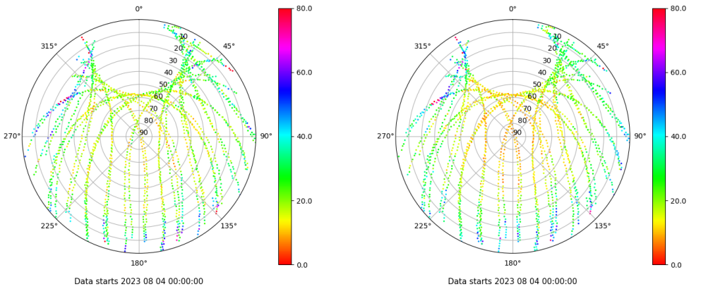
Skyplot for station YEB1. Parameter M1C Data file YEB100ESP_R_2023216.xtr Skyplot for station YEB1. Parameter M2P Data file YEB100ESP_R_2023216.xtr
