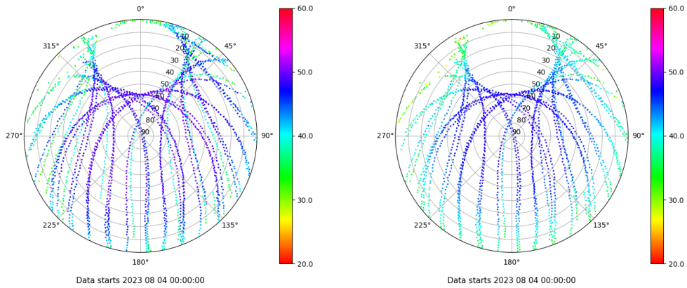
Skyplot for station YEB1. Signal to Noise S1C Data file YEB100ESP_R_2023216.xtr Skyplot for station YEB1. Signal to Noise S2P Data file YEB100ESP_R_2023216.xtr
