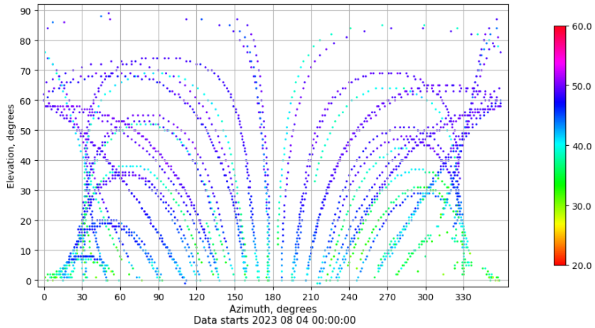
Azimuth-elevation plot for station YEB1. Signal to Noise S1C Data file YEB100ESP_R_2023216.xtr
