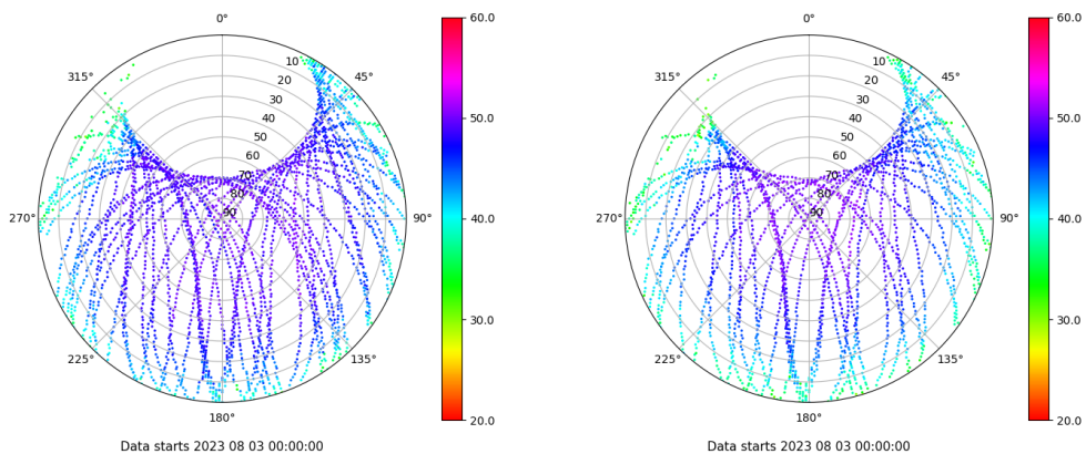
Skyplot for station YEB1. Signal to Noise S1C Data file YEB100ESP_R_2023215.xtr Skyplot for station YEB1. Signal to Noise S2S Data file YEB100ESP_R_2023215.xtr
