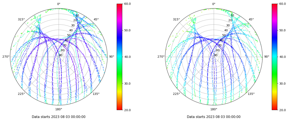
Skyplot for station YEB1. Signal to Noise S1C Data file YEB100ESP_R_2023215.xtr Skyplot for station YEB1. Signal to Noise S2P Data file YEB100ESP_R_2023215.xtr
