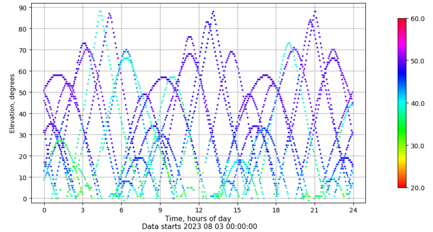
Time-elevation plot for station YEB1. Signal to Noise S1C Data file YEB100ESP_R_2023215.xtr
