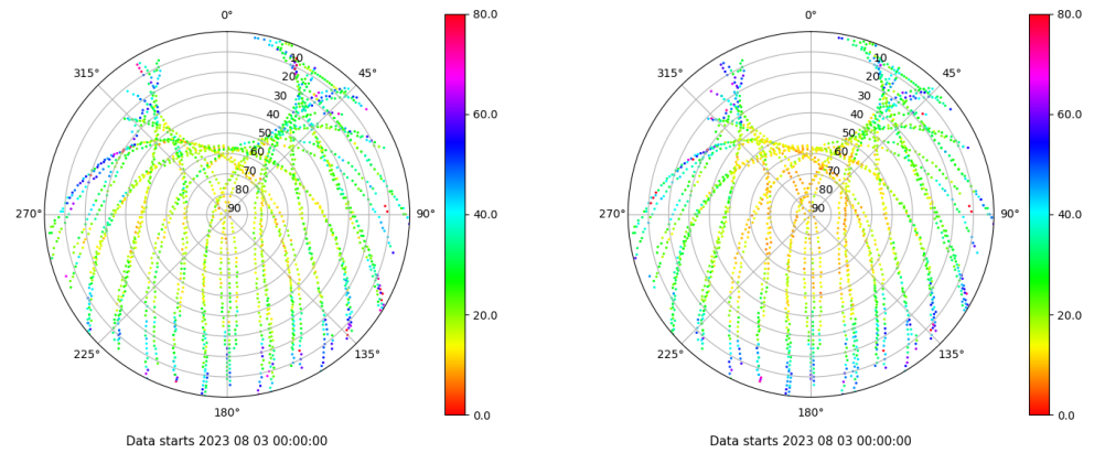
Skyplot for station YEB1. Parameter M1C Data file YEB100ESP_R_2023215.xtr Skyplot for station YEB1. Parameter M2P Data file YEB100ESP_R_2023215.xtr
