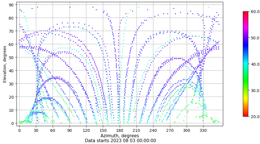
Azimuth-elevation plot for station YEB1. Signal to Noise S1C Data file YEB100ESP_R_2023215.xtr
