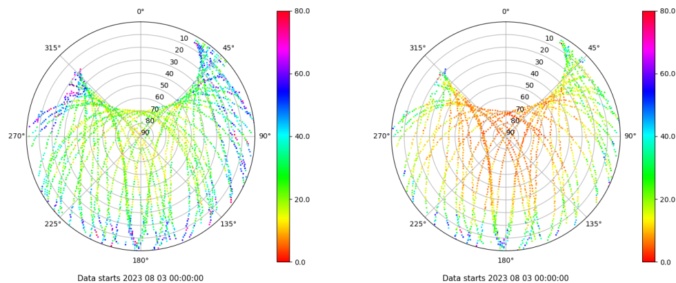
Skyplot for station YEB1. Parameter M1C Data file YEB100ESP_R_2023215.xtr Skyplot for station YEB1. Parameter M2S Data file YEB100ESP_R_2023215.xtr
