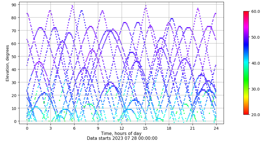
Time-elevation plot for station YEB1. Signal to Noise S1C Data file YEB100ESP_R_2023209.xtr
