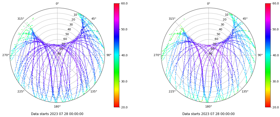
Skyplot for station YEB1. Signal to Noise S1C Data file YEB100ESP_R_2023209.xtr Skyplot for station YEB1. Signal to Noise S2S Data file YEB100ESP_R_2023209.xtr
