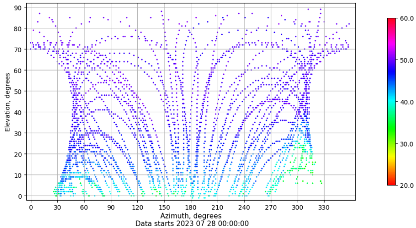
Azimuth-elevation plot for station YEB1. Signal to Noise S1C Data file YEB100ESP_R_2023209.xtr
