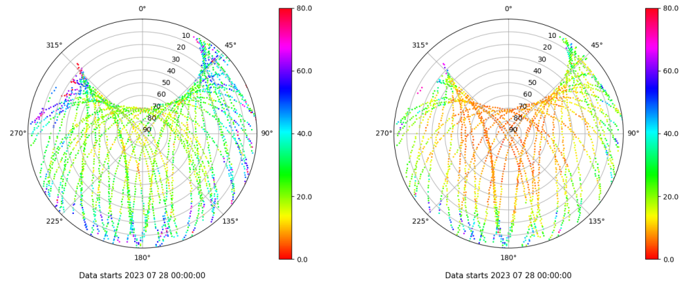
Skyplot for station YEB1. Parameter M1C Data file YEB100ESP_R_2023209.xtr Skyplot for station YEB1. Parameter M2S Data file YEB100ESP_R_2023209.xtr
