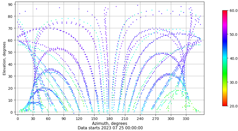
Azimuth-elevation plot for station YEB1. Signal to Noise S1C Data file YEB100ESP_R_2023206.xtr
