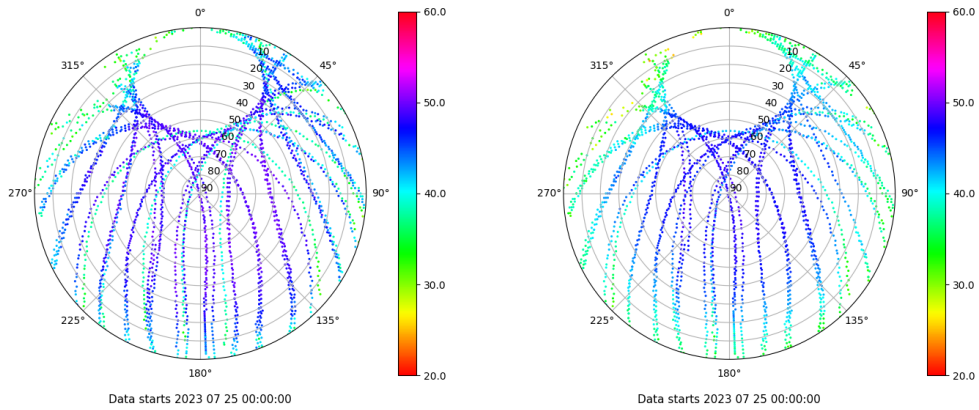
Skyplot for station YEB1. Signal to Noise S1C Data file YEB100ESP_R_2023206.xtr Skyplot for station YEB1. Signal to Noise S2P Data file YEB100ESP_R_2023206.xtr
