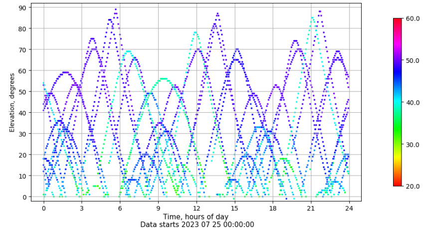
Time-elevation plot for station YEB1. Signal to Noise S1C Data file YEB100ESP_R_2023206.xtr
