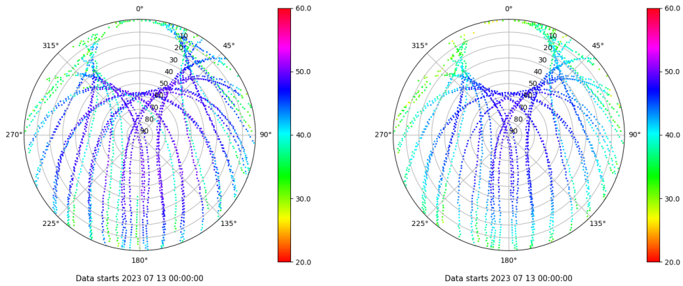
Skyplot for station YEB1. Signal to Noise S1C Data file YEB100ESP_R_2023194.xtr Skyplot for station YEB1. Signal to Noise S2P Data file YEB100ESP_R_2023194.xtr
