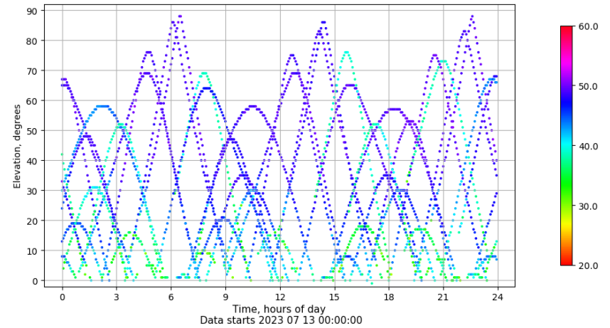
Time-elevation plot for station YEB1. Signal to Noise S1C Data file YEB100ESP_R_2023194.xtr
