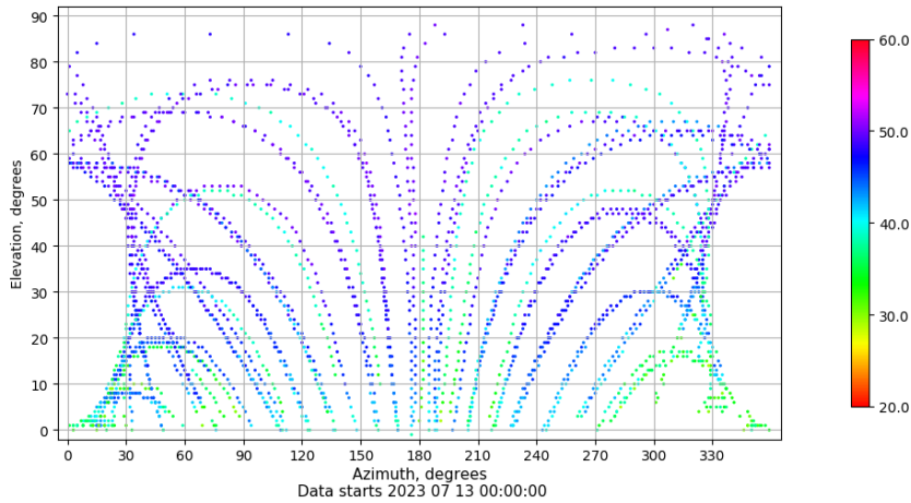
Azimuth-elevation plot for station YEB1. Signal to Noise S1C Data file YEB100ESP_R_2023194.xtr
