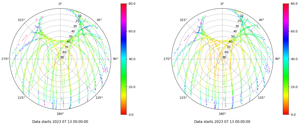
Skyplot for station YEB1. Parameter M1C Data file YEB100ESP_R_2023194.xtr Skyplot for station YEB1. Parameter M2P Data file YEB100ESP_R_2023194.xtr
