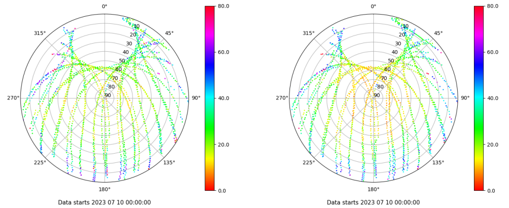
Skyplot for station YEB1. Parameter M1C Data file YEB100ESP_R_2023191.xtr Skyplot for station YEB1. Parameter M2P Data file YEB100ESP_R_2023191.xtr
