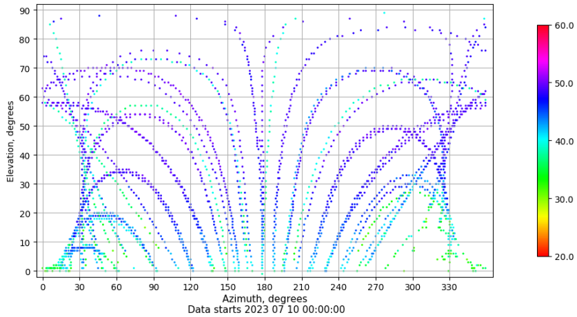
Azimuth-elevation plot for station YEB1. Signal to Noise S1C Data file YEB100ESP_R_2023191.xtr
