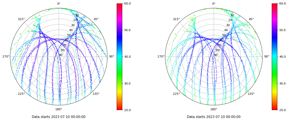
Skyplot for station YEB1. Signal to Noise S1C Data file YEB100ESP_R_2023191.xtr Skyplot for station YEB1. Signal to Noise S2P Data file YEB100ESP_R_2023191.xtr
