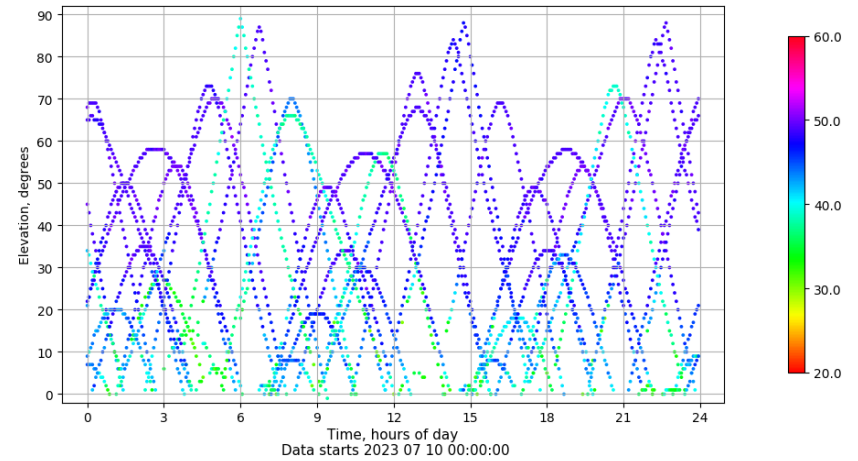
Time-elevation plot for station YEB1. Signal to Noise S1C Data file YEB100ESP_R_2023191.xtr
