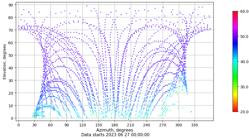
Azimuth-elevation plot for station YEB1. Signal to Noise S1C Data file YEB100ESP_R_2023178.xtr
