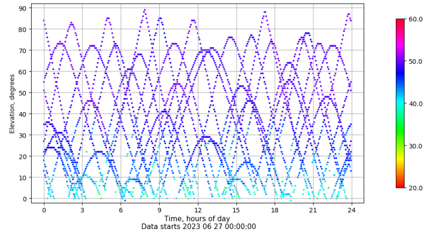
Time-elevation plot for station YEB1. Signal to Noise S1C Data file YEB100ESP_R_2023178.xtr
