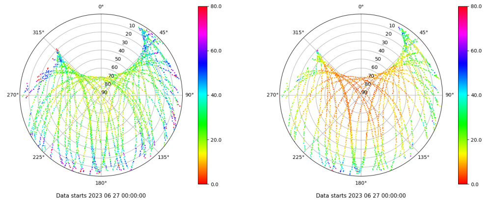
Skyplot for station YEB1. Parameter M1C Data file YEB100ESP_R_2023178.xtr Skyplot for station YEB1. Parameter M2S Data file YEB100ESP_R_2023178.xtr
