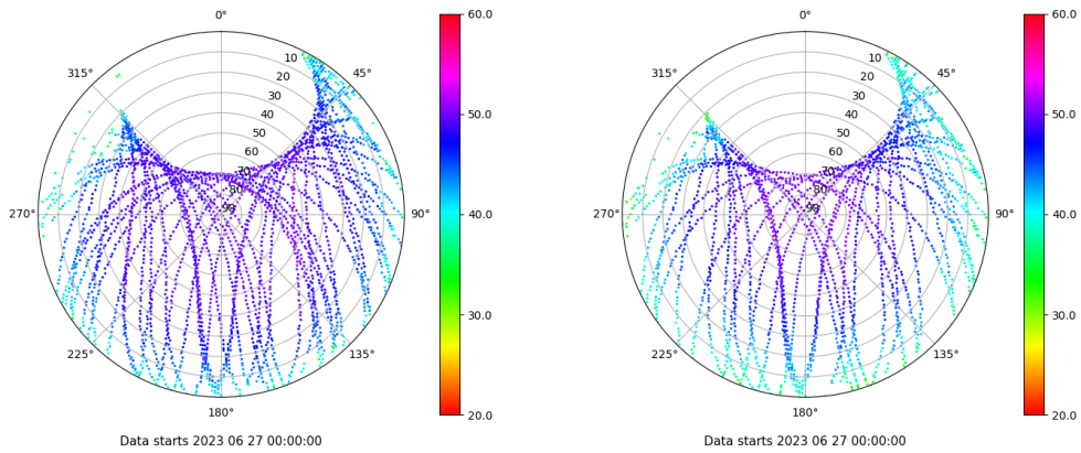
Skyplot for station YEB1. Signal to Noise S1C Data file YEB100ESP_R_2023178.xtr Skyplot for station YEB1. Signal to Noise S2S Data file YEB100ESP_R_2023178.xtr
