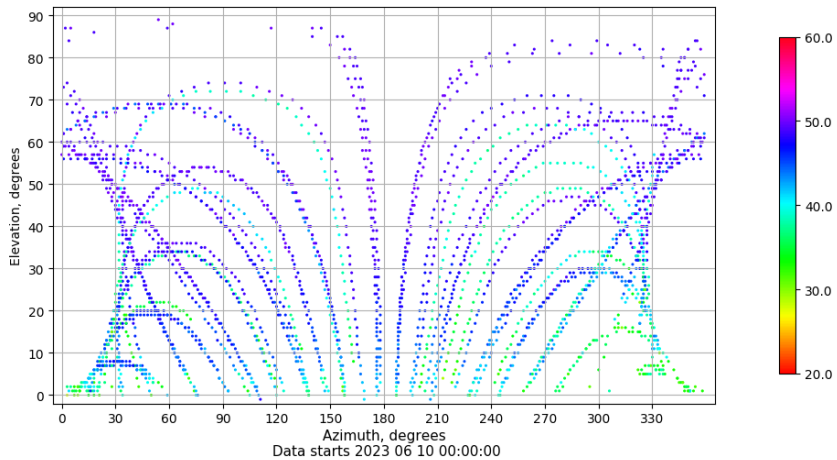
Azimuth-elevation plot for station YEB1. Signal to Noise S1C Data file YEB100ESP_R_2023161.xtr
