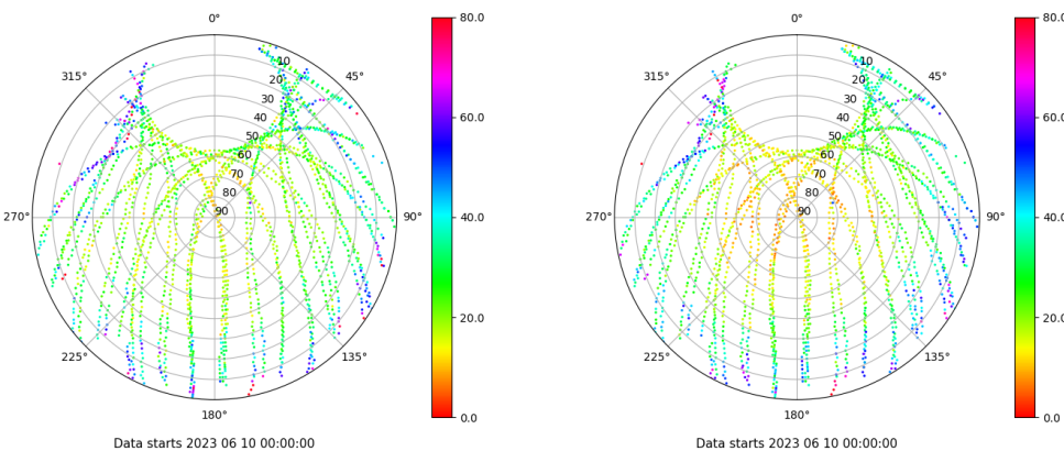
Skyplot for station YEB1. Parameter M1C Data file YEB100ESP_R_2023161.xtr Skyplot for station YEB1. Parameter M2P Data file YEB100ESP_R_2023161.xtr
