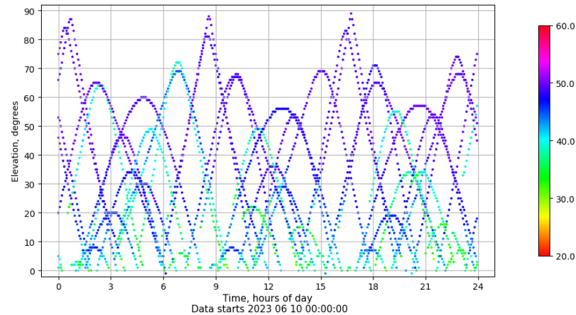
Time-elevation plot for station YEB1. Signal to Noise S1C Data file YEB100ESP_R_2023161.xtr
