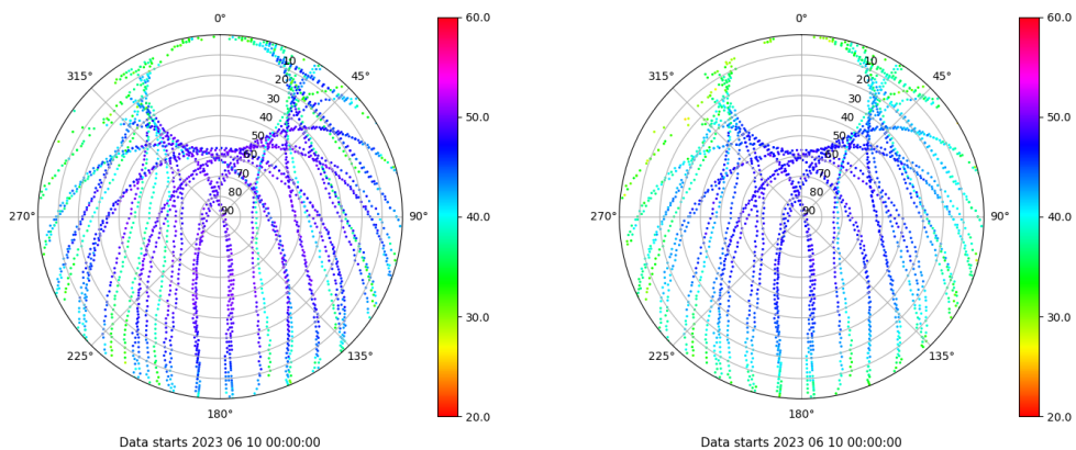
Skyplot for station YEB1. Signal to Noise S1C Data file YEB100ESP_R_2023161.xtr Skyplot for station YEB1. Signal to Noise S2P Data file YEB100ESP_R_2023161.xtr
