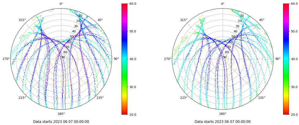
Skyplot for station YEB1. Signal to Noise S1C Data file YEB100ESP_R_2023158.xtr Skyplot for station YEB1. Signal to Noise S2P Data file YEB100ESP_R_2023158.xtr
