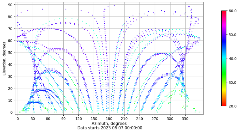
Azimuth-elevation plot for station YEB1. Signal to Noise S1C Data file YEB100ESP_R_2023158.xtr
