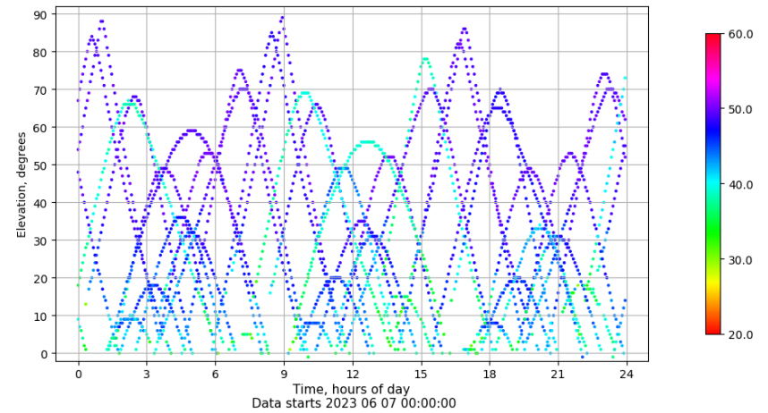
Time-elevation plot for station YEB1. Signal to Noise S1C Data file YEB100ESP_R_2023158.xtr
