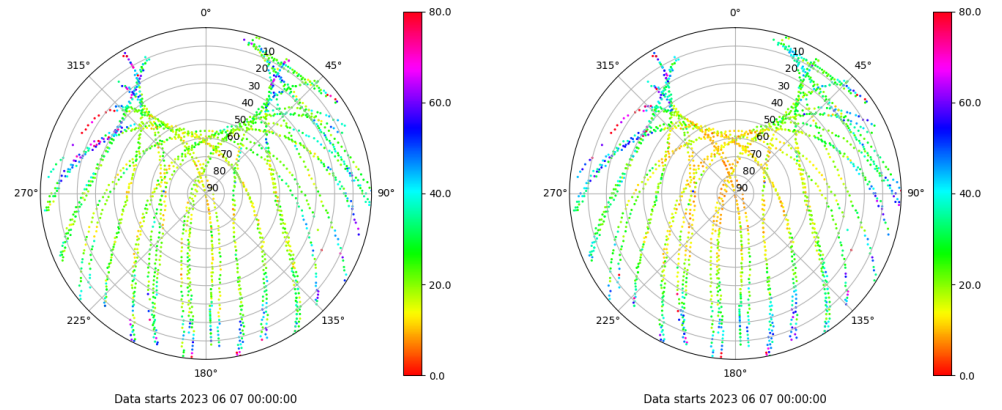
Skyplot for station YEB1. Parameter M1C Data file YEB100ESP_R_2023158.xtr Skyplot for station YEB1. Parameter M2P Data file YEB100ESP_R_2023158.xtr
