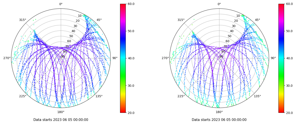
Skyplot for station YEB1. Signal to Noise S1C Data file YEB100ESP_R_2023156.xtr Skyplot for station YEB1. Signal to Noise S2S Data file YEB100ESP_R_2023156.xtr
