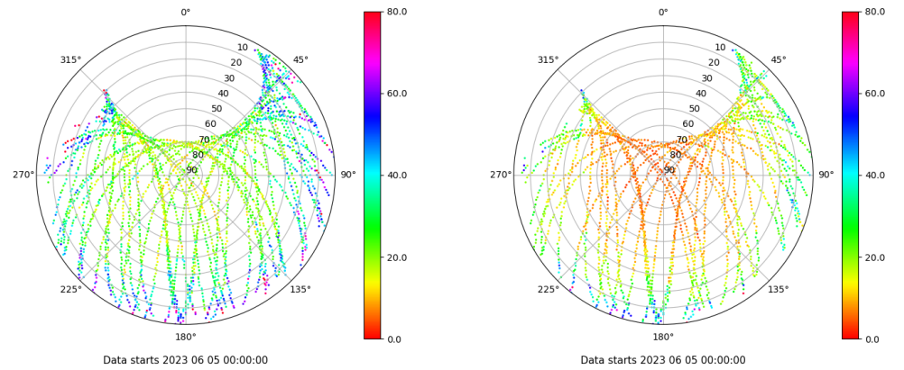
Skyplot for station YEB1. Parameter M1C Data file YEB100ESP_R_2023156.xtr Skyplot for station YEB1. Parameter M2S Data file YEB100ESP_R_2023156.xtr
