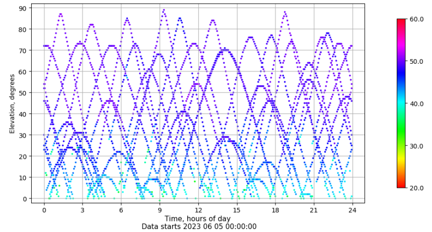
Time-elevation plot for station YEB1. Signal to Noise S1C Data file YEB100ESP_R_2023156.xtr
