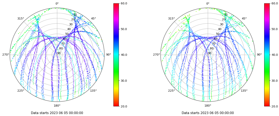
Skyplot for station YEB1. Signal to Noise S1C Data file YEB100ESP_R_2023156.xtr Skyplot for station YEB1. Signal to Noise S2P Data file YEB100ESP_R_2023156.xtr
