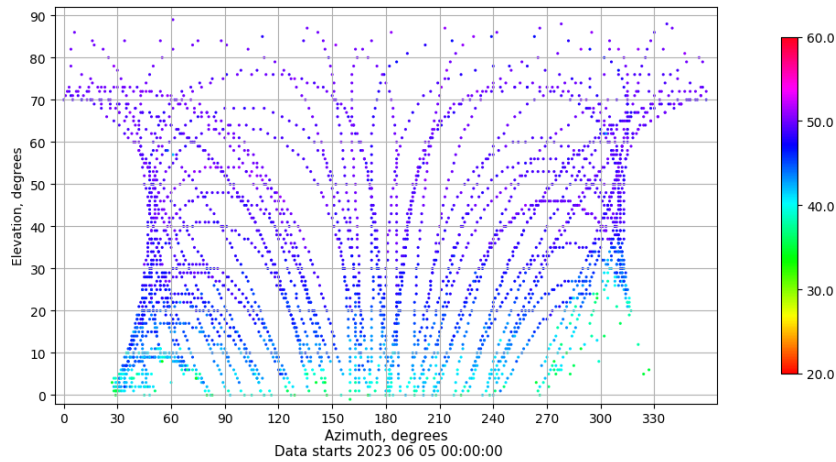
Azimuth-elevation plot for station YEB1. Signal to Noise S1C Data file YEB100ESP_R_2023156.xtr
