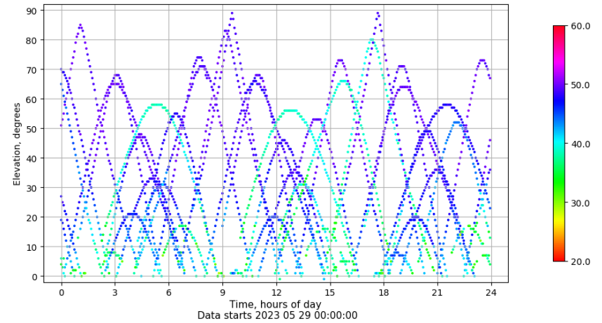
Time-elevation plot for station YEB1. Signal to Noise S1C Data file YEB100ESP_R_2023149.xtr
