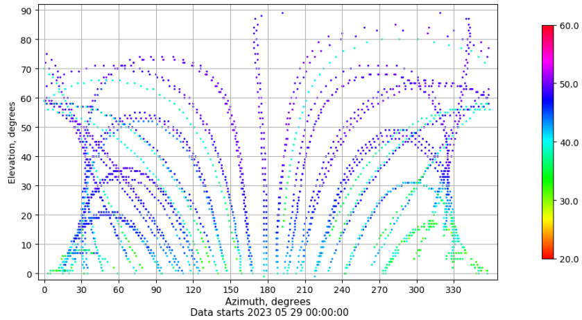
Azimuth-elevation plot for station YEB1. Signal to Noise S1C Data file YEB100ESP_R_2023149.xtr
