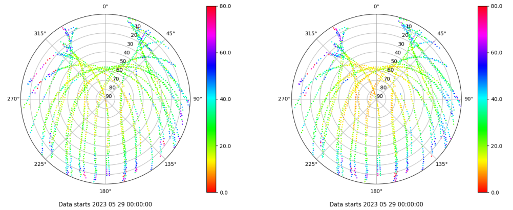
Skyplot for station YEB1. Parameter M1C Data file YEB100ESP_R_2023149.xtr Skyplot for station YEB1. Parameter M2P Data file YEB100ESP_R_2023149.xtr
