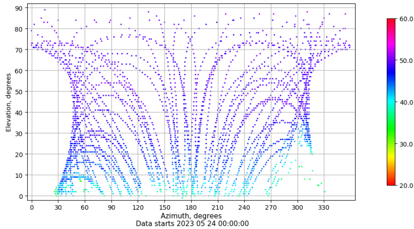
Azimuth-elevation plot for station YEB1. Signal to Noise S1C Data file YEB100ESP_R_2023144.xtr
