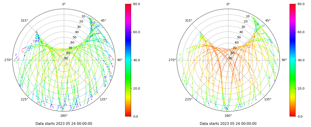
Skyplot for station YEB1. Parameter M1C Data file YEB100ESP_R_2023144.xtr Skyplot for station YEB1. Parameter M2S Data file YEB100ESP_R_2023144.xtr
