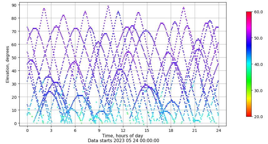
Time-elevation plot for station YEB1. Signal to Noise S1C Data file YEB100ESP_R_2023144.xtr
