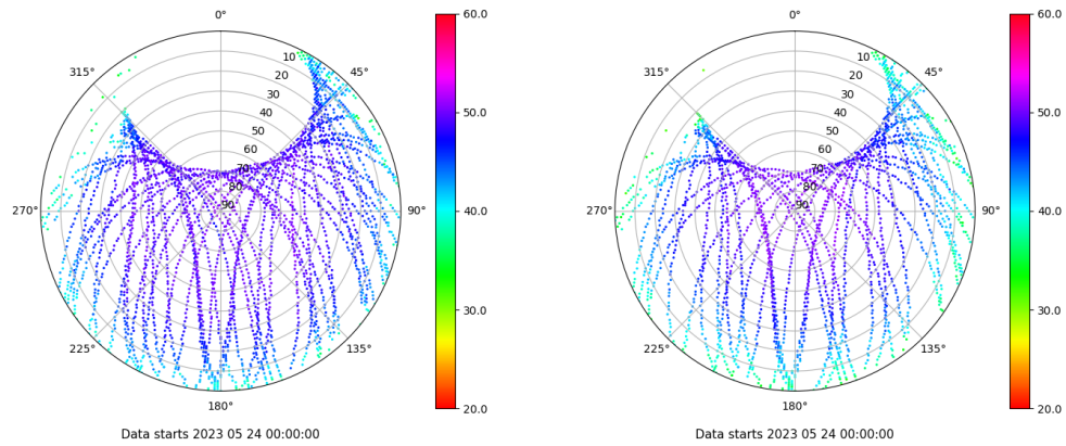
Skyplot for station YEB1. Signal to Noise S1C Data file YEB100ESP_R_2023144.xtr Skyplot for station YEB1. Signal to Noise S2S Data file YEB100ESP_R_2023144.xtr
