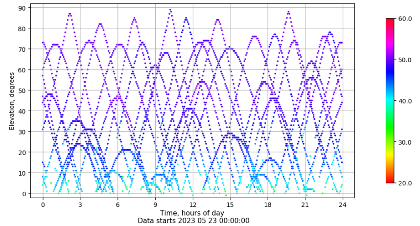
Time-elevation plot for station YEB1. Signal to Noise S1C Data file YEB100ESP_R_2023143.xtr
