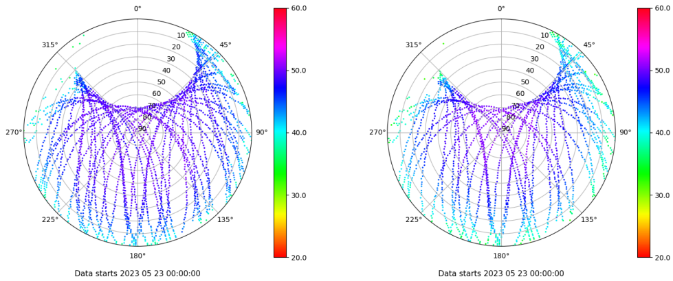
Skyplot for station YEB1. Signal to Noise S1C Data file YEB100ESP_R_2023143.xtr Skyplot for station YEB1. Signal to Noise S2S Data file YEB100ESP_R_2023143.xtr
