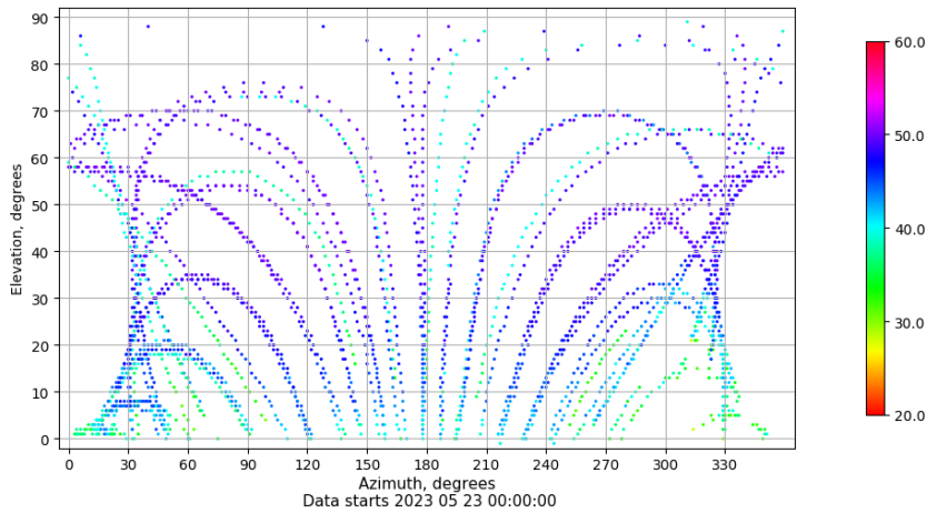
Azimuth-elevation plot for station YEB1. Signal to Noise S1C Data file YEB100ESP_R_2023143.xtr
