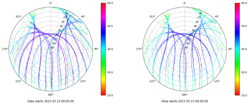
Skyplot for station YEB1. Signal to Noise S1C Data file YEB100ESP_R_2023143.xtr Skyplot for station YEB1. Signal to Noise S2P Data file YEB100ESP_R_2023143.xtr
