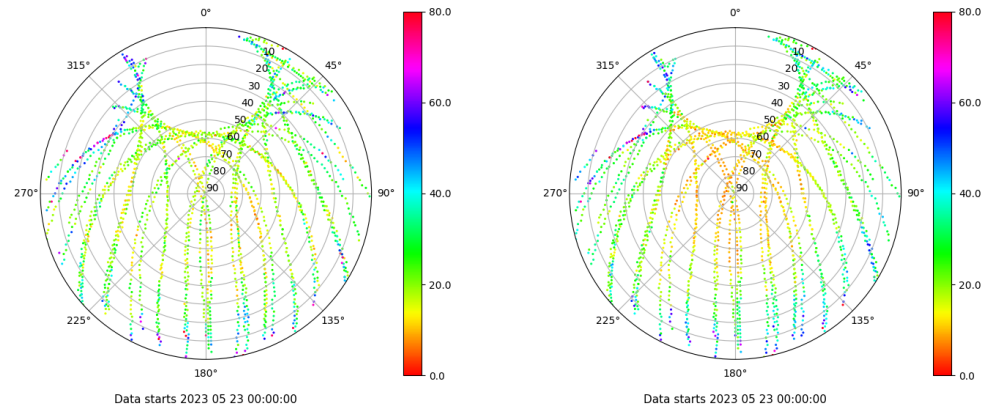
Skyplot for station YEB1. Parameter M1C Data file YEB100ESP_R_2023143.xtr Skyplot for station YEB1. Parameter M2P Data file YEB100ESP_R_2023143.xtr
