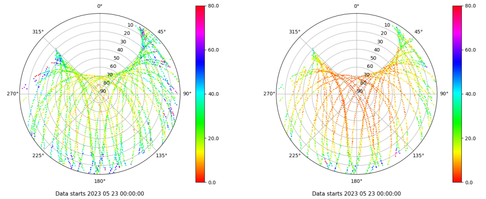
Skyplot for station YEB1. Parameter M1C Data file YEB100ESP_R_2023143.xtr Skyplot for station YEB1. Parameter M2S Data file YEB100ESP_R_2023143.xtr
