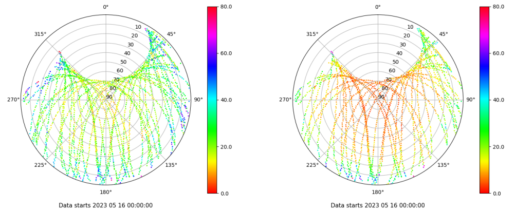
Skyplot for station YEB1. Parameter M1C Data file YEB100ESP_R_2023136.xtr Skyplot for station YEB1. Parameter M2S Data file YEB100ESP_R_2023136.xtr
