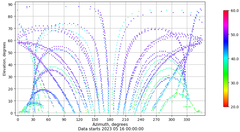
Azimuth-elevation plot for station YEB1. Signal to Noise S1C Data file YEB100ESP_R_2023136.xtr
