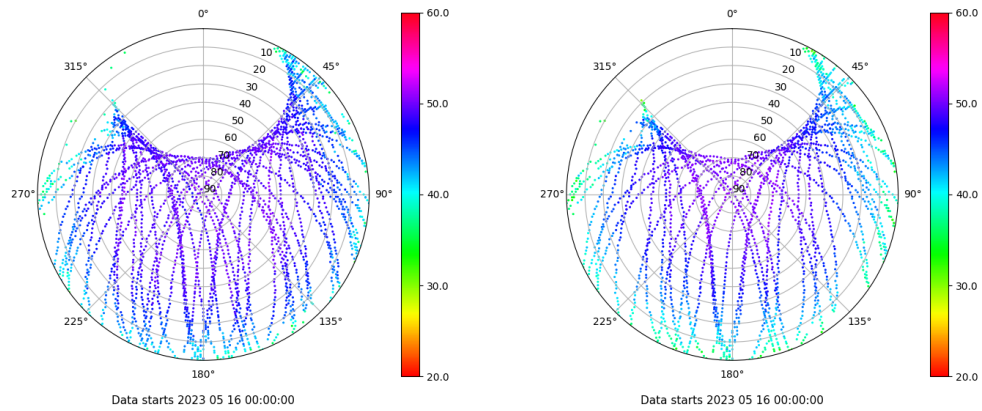
Skyplot for station YEB1. Signal to Noise S1C Data file YEB100ESP_R_2023136.xtr Skyplot for station YEB1. Signal to Noise S2S Data file YEB100ESP_R_2023136.xtr
