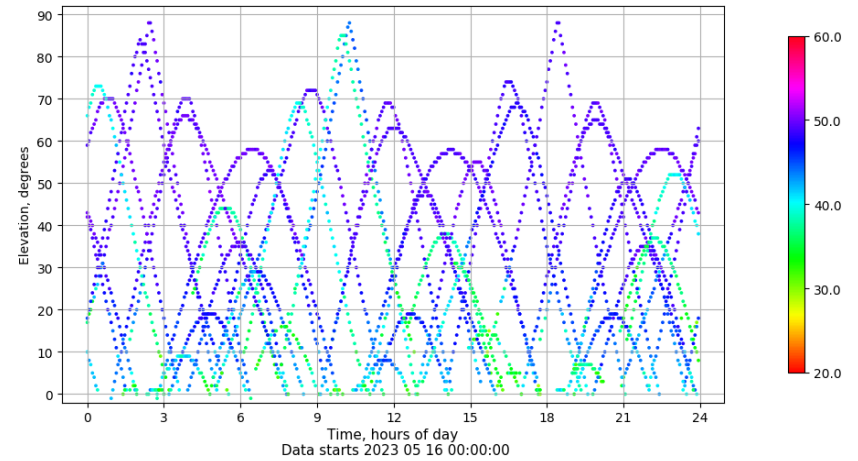
Time-elevation plot for station YEB1. Signal to Noise S1C Data file YEB100ESP_R_2023136.xtr
