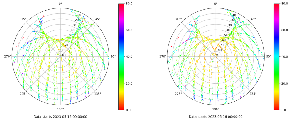
Skyplot for station YEB1. Parameter M1C Data file YEB100ESP_R_2023136.xtr Skyplot for station YEB1. Parameter M2P Data file YEB100ESP_R_2023136.xtr
