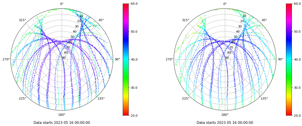
Skyplot for station YEB1. Signal to Noise S1C Data file YEB100ESP_R_2023136.xtr Skyplot for station YEB1. Signal to Noise S2P Data file YEB100ESP_R_2023136.xtr
