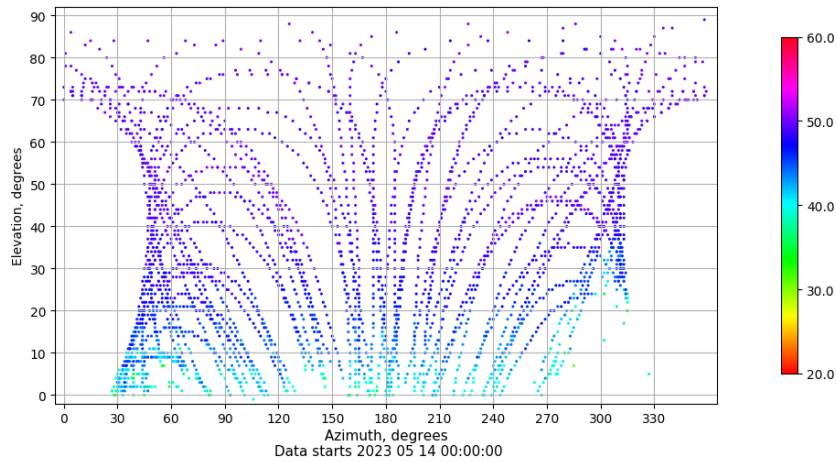
Azimuth-elevation plot for station YEB1. Signal to Noise S1C Data file YEB100ESP_R_2023134.xtr
