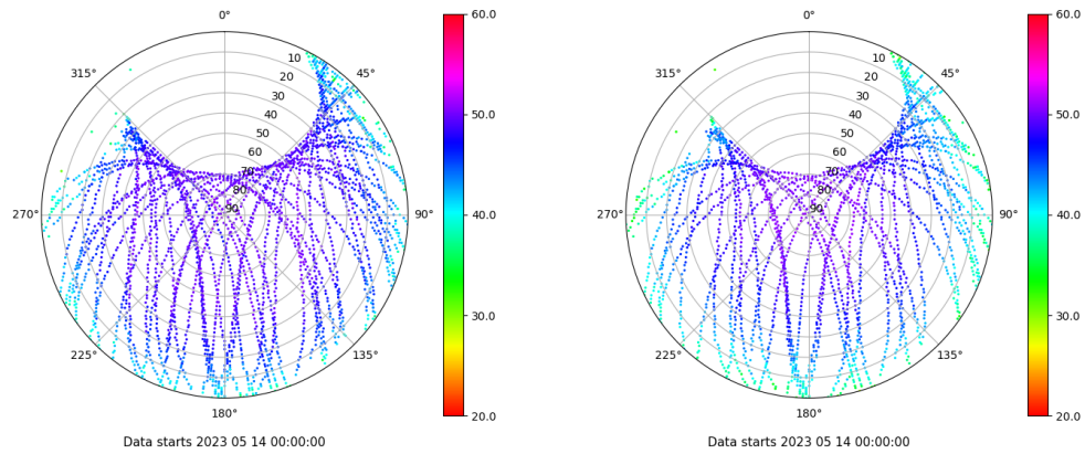
Skyplot for station YEB1. Signal to Noise S1C Data file YEB100ESP_R_2023134.xtr Skyplot for station YEB1. Signal to Noise S2S Data file YEB100ESP_R_2023134.xtr
