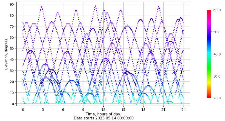
Time-elevation plot for station YEB1. Signal to Noise S1C Data file YEB100ESP_R_2023134.xtr
