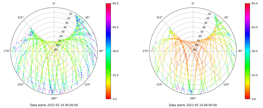
Skyplot for station YEB1. Parameter M1C Data file YEB100ESP_R_2023134.xtr Skyplot for station YEB1. Parameter M2S Data file YEB100ESP_R_2023134.xtr
