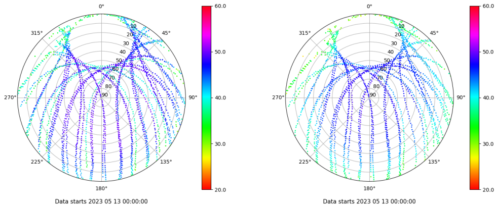
Skyplot for station YEB1. Signal to Noise S1C Data file YEB100ESP_R_2023133.xtr Skyplot for station YEB1. Signal to Noise S2P Data file YEB100ESP_R_2023133.xtr
