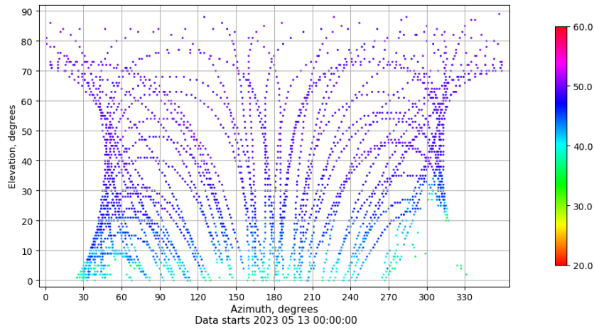
Azimuth-elevation plot for station YEB1. Signal to Noise S1C Data file YEB100ESP_R_2023133.xtr
