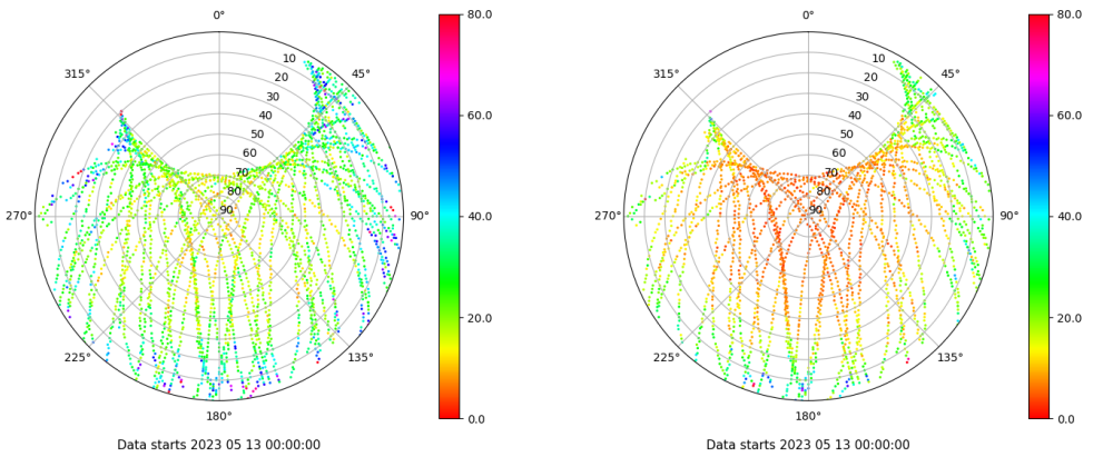
Skyplot for station YEB1. Parameter M1C Data file YEB100ESP_R_2023133.xtr Skyplot for station YEB1. Parameter M2S Data file YEB100ESP_R_2023133.xtr
