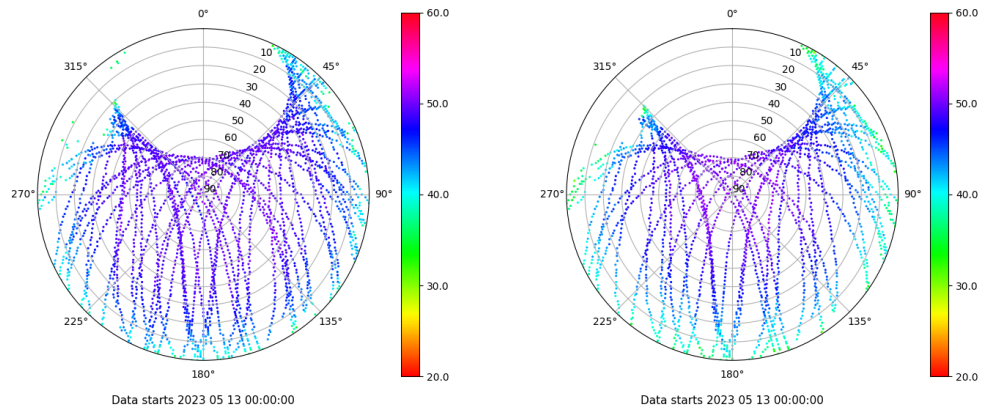
Skyplot for station YEB1. Signal to Noise S1C Data file YEB100ESP_R_2023133.xtr Skyplot for station YEB1. Signal to Noise S2S Data file YEB100ESP_R_2023133.xtr
