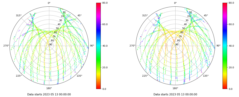
Skyplot for station YEB1. Parameter M1C Data file YEB100ESP_R_2023133.xtr Skyplot for station YEB1. Parameter M2P Data file YEB100ESP_R_2023133.xtr
