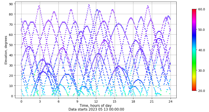
Time-elevation plot for station YEB1. Signal to Noise S1C Data file YEB100ESP_R_2023133.xtr
