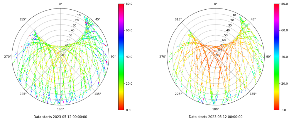
Skyplot for station YEB1. Parameter M1C Data file YEB100ESP_R_2023132.xtr Skyplot for station YEB1. Parameter M2S Data file YEB100ESP_R_2023132.xtr
