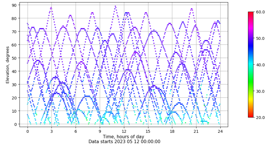
Time-elevation plot for station YEB1. Signal to Noise S1C Data file YEB100ESP_R_2023132.xtr
