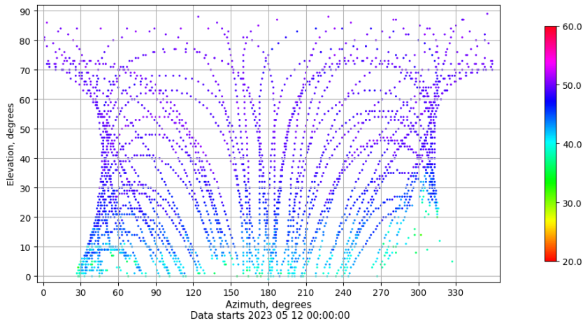
Azimuth-elevation plot for station YEB1. Signal to Noise S1C Data file YEB100ESP_R_2023132.xtr
