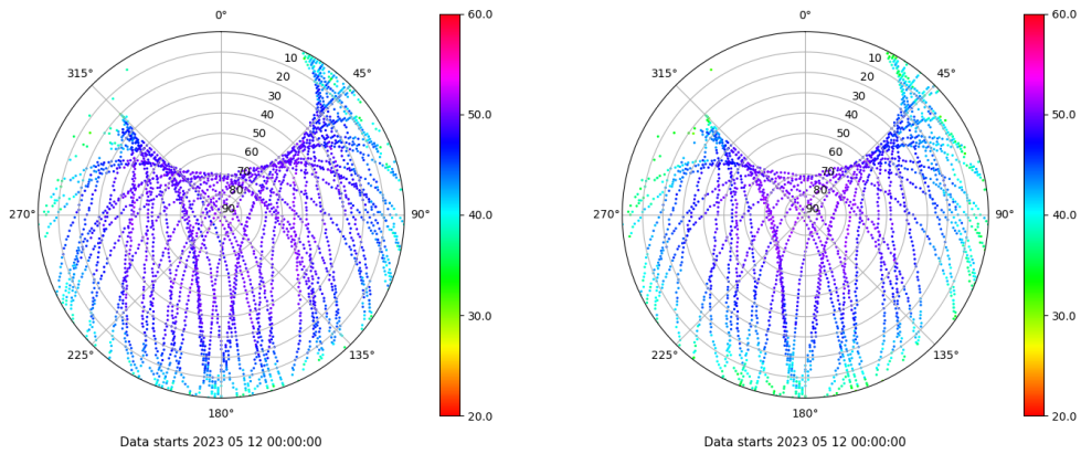
Skyplot for station YEB1. Signal to Noise S1C Data file YEB100ESP_R_2023132.xtr Skyplot for station YEB1. Signal to Noise S2S Data file YEB100ESP_R_2023132.xtr
