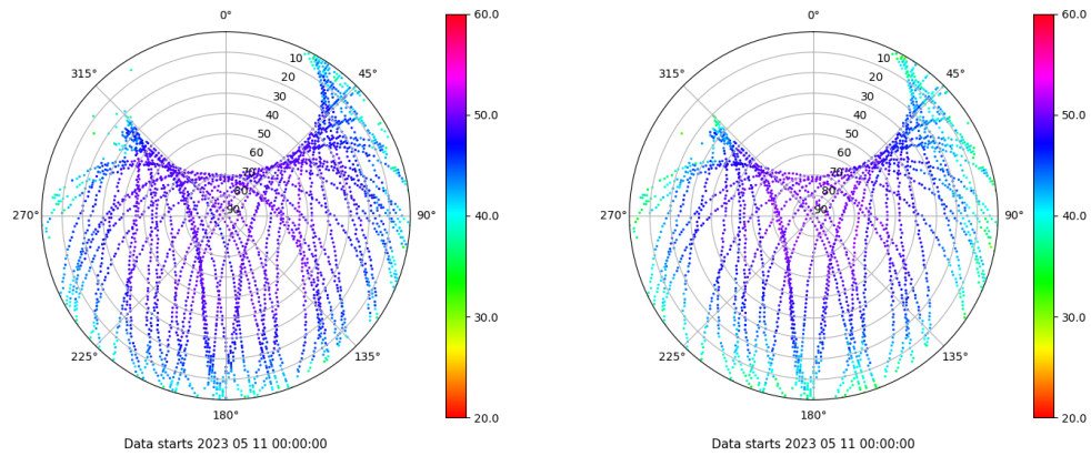
Skyplot for station YEB1. Signal to Noise S1C Data file YEB100ESP_R_2023131.xtr Skyplot for station YEB1. Signal to Noise S2S Data file YEB100ESP_R_2023131.xtr
