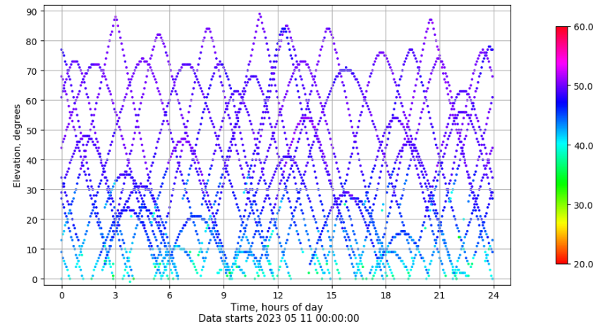
Time-elevation plot for station YEB1. Signal to Noise S1C Data file YEB100ESP_R_2023131.xtr
