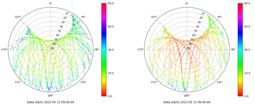
Skyplot for station YEB1. Parameter M1C Data file YEB100ESP_R_2023131.xtr Skyplot for station YEB1. Parameter M2S Data file YEB100ESP_R_2023131.xtr
