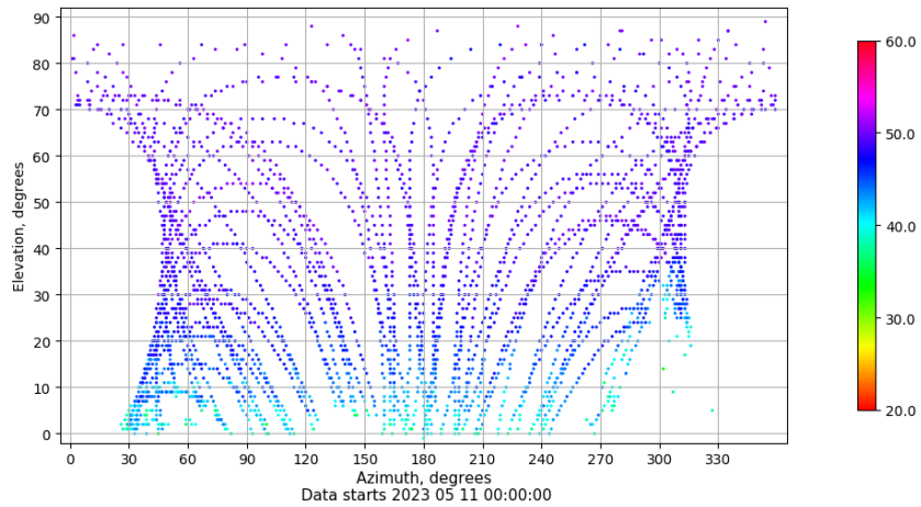
Azimuth-elevation plot for station YEB1. Signal to Noise S1C Data file YEB100ESP_R_2023131.xtr
