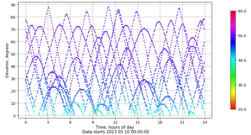
Time-elevation plot for station YEB1. Signal to Noise S1C Data file YEB100ESP_R_2023130.xtr
