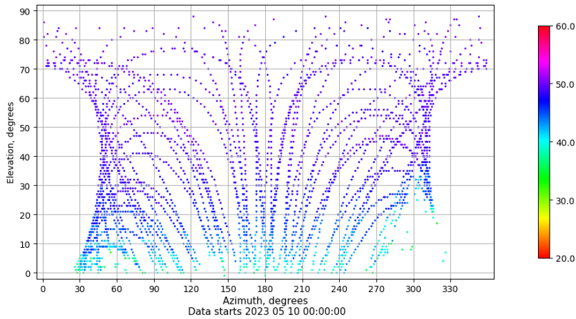
Azimuth-elevation plot for station YEB1. Signal to Noise S1C Data file YEB100ESP_R_2023130.xtr
