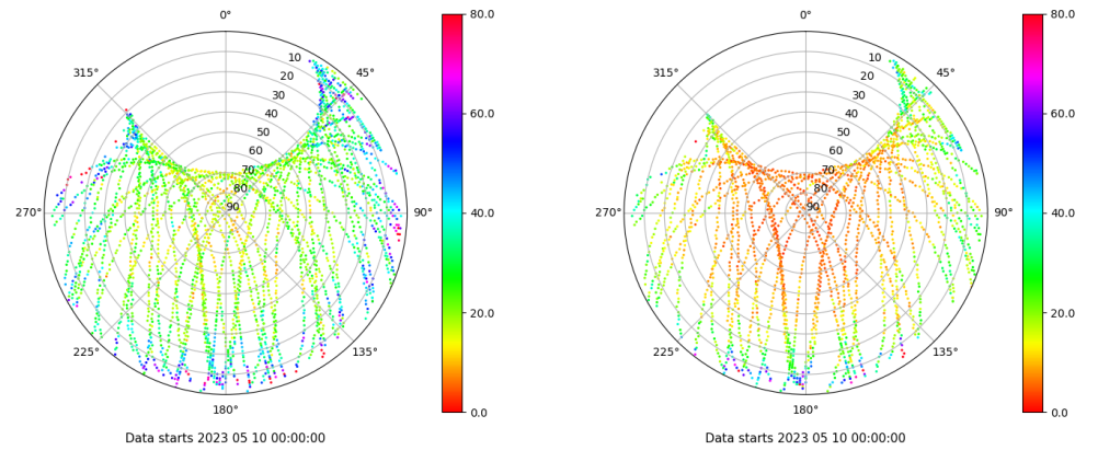
Skyplot for station YEB1. Parameter M1C Data file YEB100ESP_R_2023130.xtr Skyplot for station YEB1. Parameter M2S Data file YEB100ESP_R_2023130.xtr
