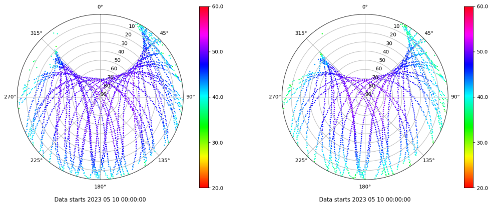
Skyplot for station YEB1. Signal to Noise S1C Data file YEB100ESP_R_2023130.xtr Skyplot for station YEB1. Signal to Noise S2S Data file YEB100ESP_R_2023130.xtr
