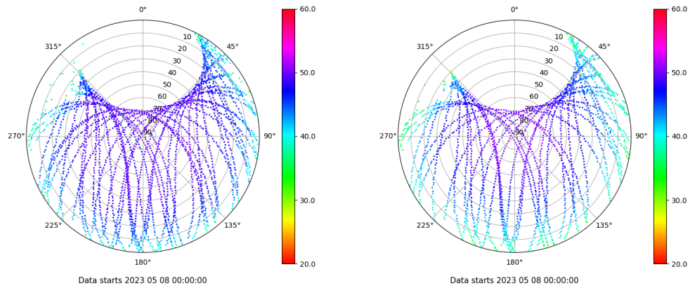
Skyplot for station YEB1. Signal to Noise S1C Data file YEB100ESP_R_2023128.xtr Skyplot for station YEB1. Signal to Noise S2S Data file YEB100ESP_R_2023128.xtr
