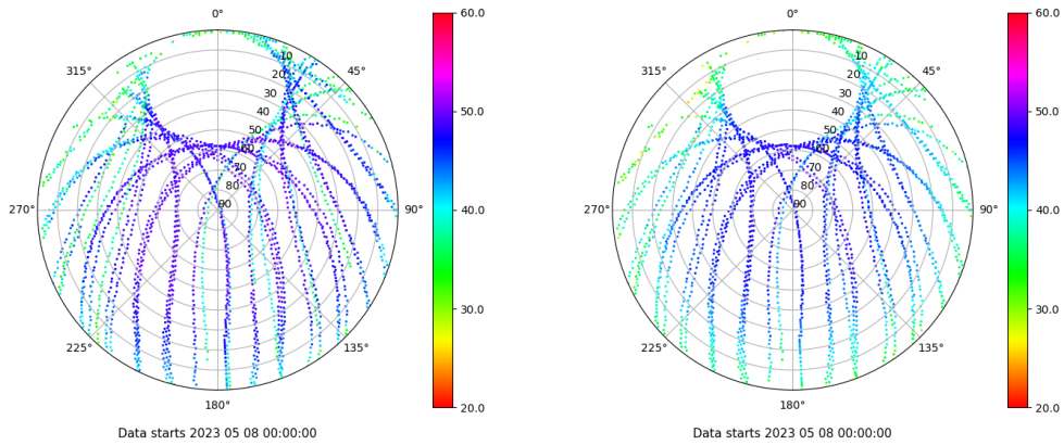
Skyplot for station YEB1. Signal to Noise S1C Data file YEB100ESP_R_2023128.xtr Skyplot for station YEB1. Signal to Noise S2P Data file YEB100ESP_R_2023128.xtr
