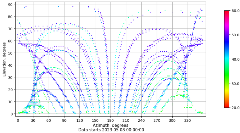
Azimuth-elevation plot for station YEB1. Signal to Noise S1C Data file YEB100ESP_R_2023128.xtr
