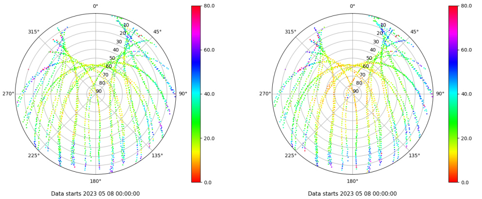
Skyplot for station YEB1. Parameter M1C Data file YEB100ESP_R_2023128.xtr Skyplot for station YEB1. Parameter M2P Data file YEB100ESP_R_2023128.xtr
