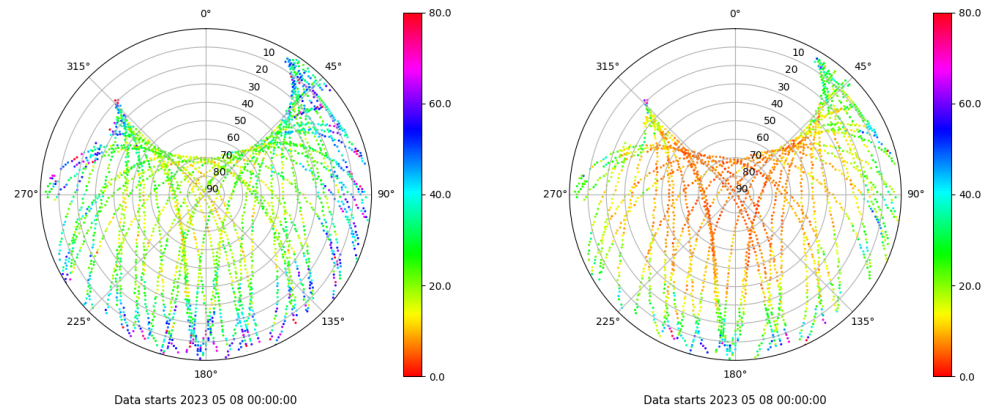
Skyplot for station YEB1. Parameter M1C Data file YEB100ESP_R_2023128.xtr Skyplot for station YEB1. Parameter M2S Data file YEB100ESP_R_2023128.xtr
