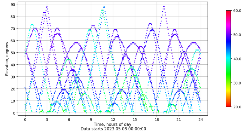
Time-elevation plot for station YEB1. Signal to Noise S1C Data file YEB100ESP_R_2023128.xtr
