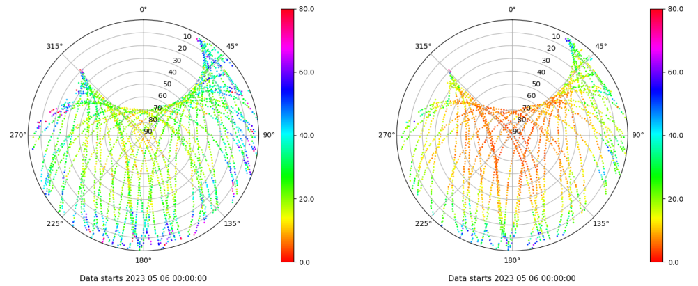
Skyplot for station YEB1. Parameter M1C Data file YEB100ESP_R_2023126.xtr Skyplot for station YEB1. Parameter M2S Data file YEB100ESP_R_2023126.xtr
