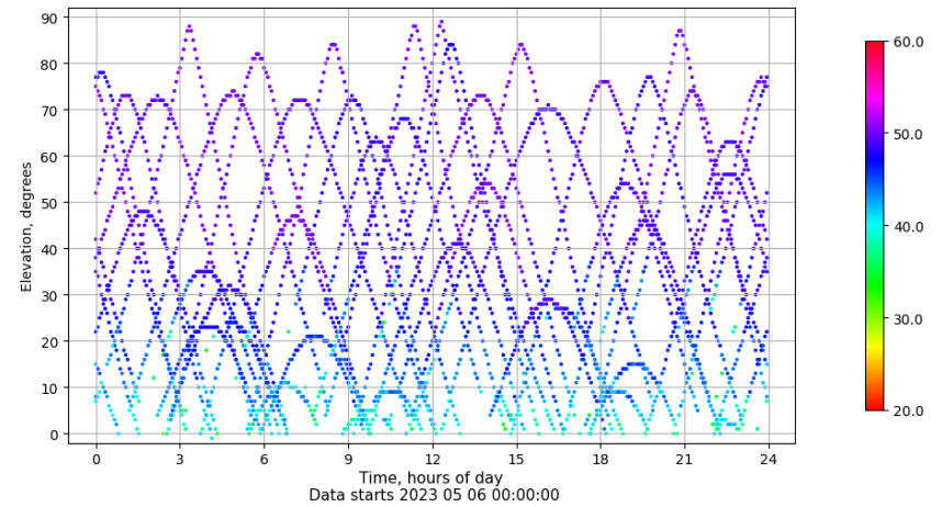
Time-elevation plot for station YEB1. Signal to Noise S1C Data file YEB100ESP_R_2023126.xtr
