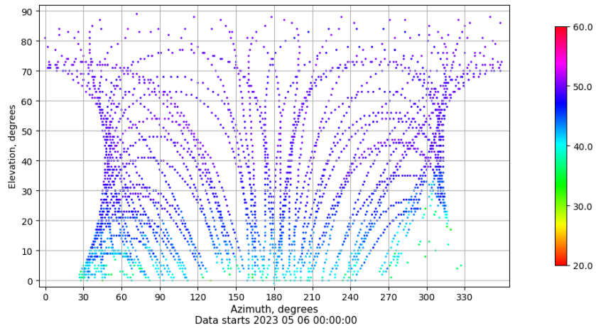
Azimuth-elevation plot for station YEB1. Signal to Noise S1C Data file YEB100ESP_R_2023126.xtr
