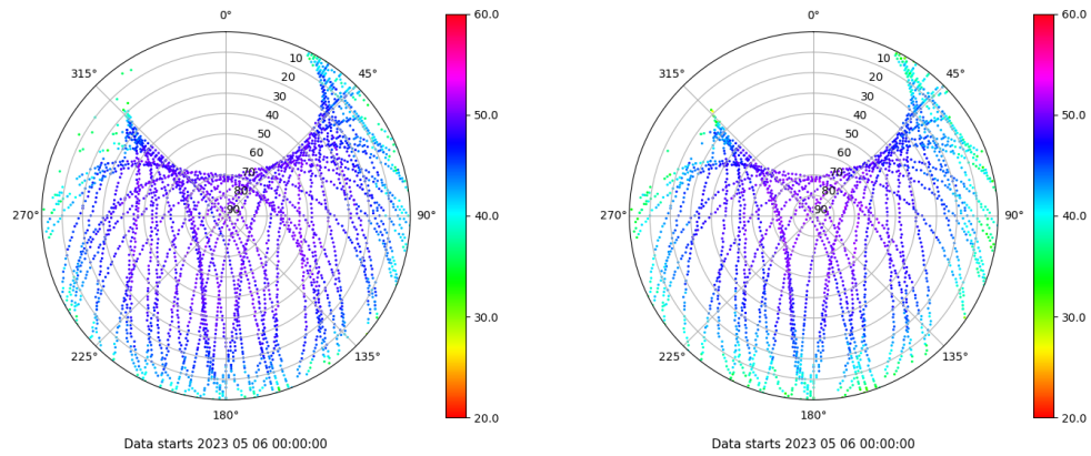
Skyplot for station YEB1. Signal to Noise S1C Data file YEB100ESP_R_2023126.xtr Skyplot for station YEB1. Signal to Noise S2S Data file YEB100ESP_R_2023126.xtr
