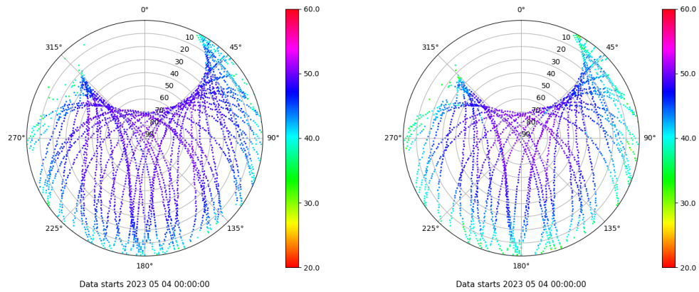
Skyplot for station YEB1. Signal to Noise S1C Data file YEB100ESP_R_2023124.xtr Skyplot for station YEB1. Signal to Noise S2S Data file YEB100ESP_R_2023124.xtr
