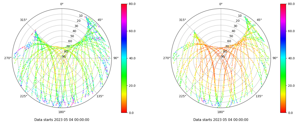
Skyplot for station YEB1. Parameter M1C Data file YEB100ESP_R_2023124.xtr Skyplot for station YEB1. Parameter M2S Data file YEB100ESP_R_2023124.xtr
