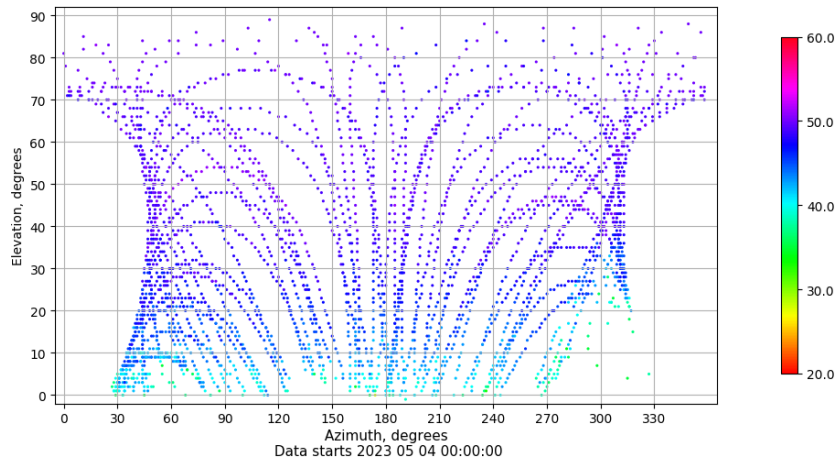
Azimuth-elevation plot for station YEB1. Signal to Noise S1C Data file YEB100ESP_R_2023124.xtr
