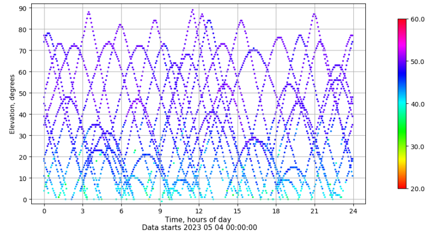
Time-elevation plot for station YEB1. Signal to Noise S1C Data file YEB100ESP_R_2023124.xtr
