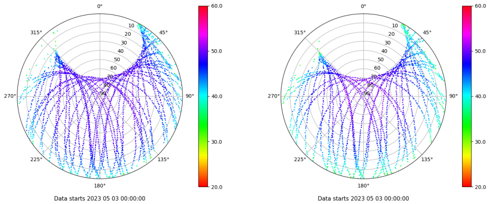
Skyplot for station YEB1. Signal to Noise S1C Data file YEB100ESP_R_2023123.xtr Skyplot for station YEB1. Signal to Noise S2S Data file YEB100ESP_R_2023123.xtr
