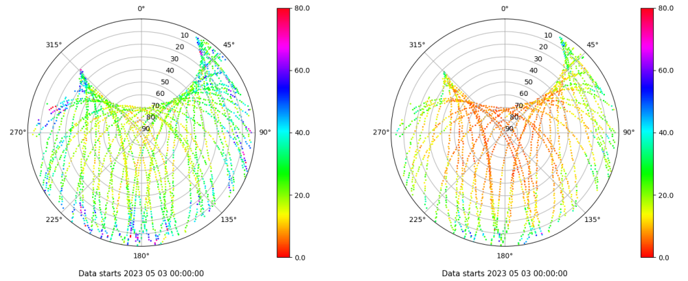
Skyplot for station YEB1. Parameter M1C Data file YEB100ESP_R_2023123.xtr Skyplot for station YEB1. Parameter M2S Data file YEB100ESP_R_2023123.xtr
