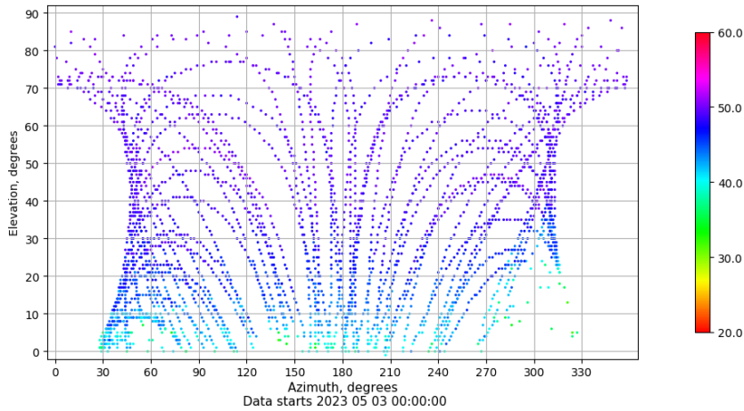
Azimuth-elevation plot for station YEB1. Signal to Noise S1C Data file YEB100ESP_R_2023123.xtr
