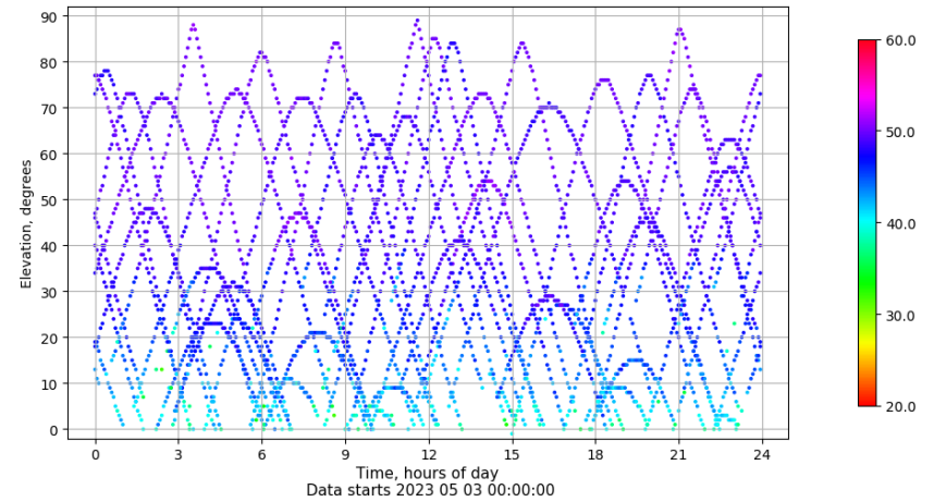
Time-elevation plot for station YEB1. Signal to Noise S1C Data file YEB100ESP_R_2023123.xtr
