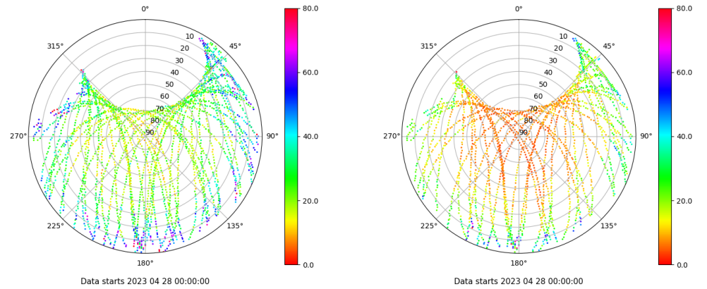
Skyplot for station YEB1. Parameter M1C Data file YEB100ESP_R_2023118.xtr Skyplot for station YEB1. Parameter M2S Data file YEB100ESP_R_2023118.xtr
