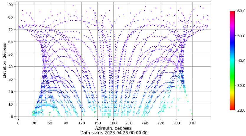
Azimuth-elevation plot for station YEB1. Signal to Noise S1C Data file YEB100ESP_R_2023118.xtr
