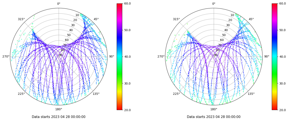
Skyplot for station YEB1. Signal to Noise S1C Data file YEB100ESP_R_2023118.xtr Skyplot for station YEB1. Signal to Noise S2S Data file YEB100ESP_R_2023118.xtr
