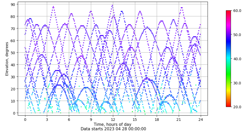
Time-elevation plot for station YEB1. Signal to Noise S1C Data file YEB100ESP_R_2023118.xtr
