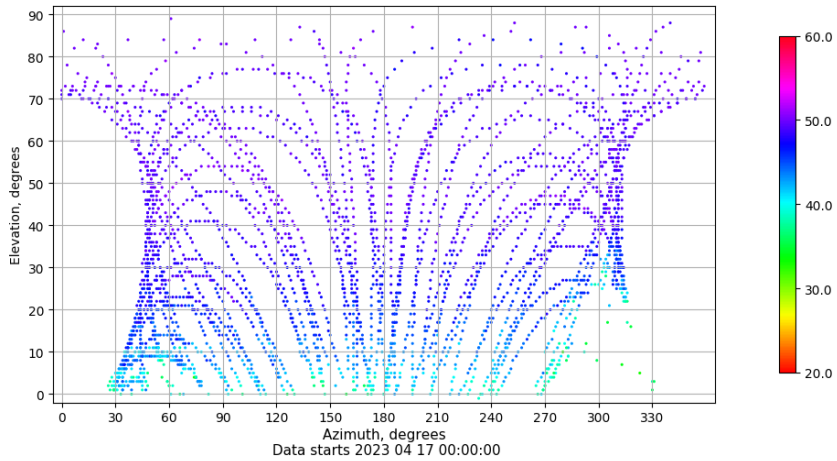
Azimuth-elevation plot for station YEB1. Signal to Noise S1C Data file YEB100ESP_R_2023107.xtr
