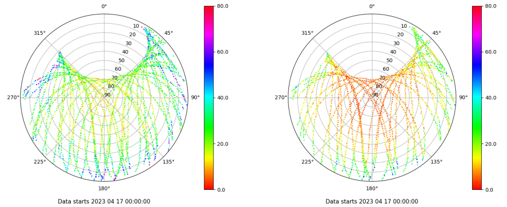
Skyplot for station YEB1. Parameter M1C Data file YEB100ESP_R_2023107.xtr Skyplot for station YEB1. Parameter M2S Data file YEB100ESP_R_2023107.xtr
