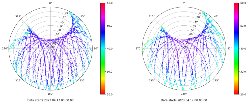
Skyplot for station YEB1. Signal to Noise S1C Data file YEB100ESP_R_2023107.xtr Skyplot for station YEB1. Signal to Noise S2S Data file YEB100ESP_R_2023107.xtr
