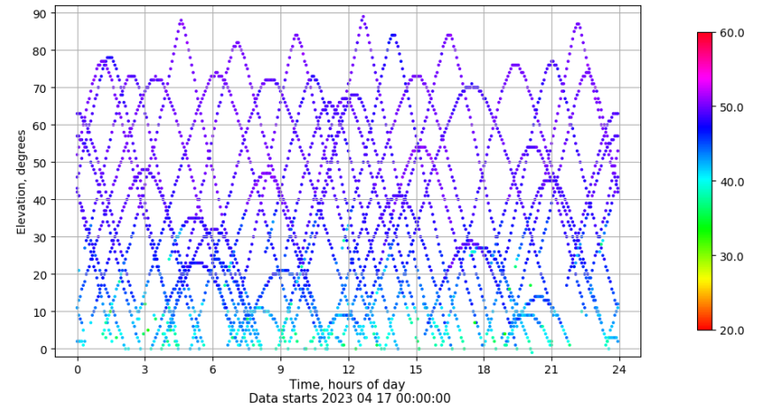
Time-elevation plot for station YEB1. Signal to Noise S1C Data file YEB100ESP_R_2023107.xtr
