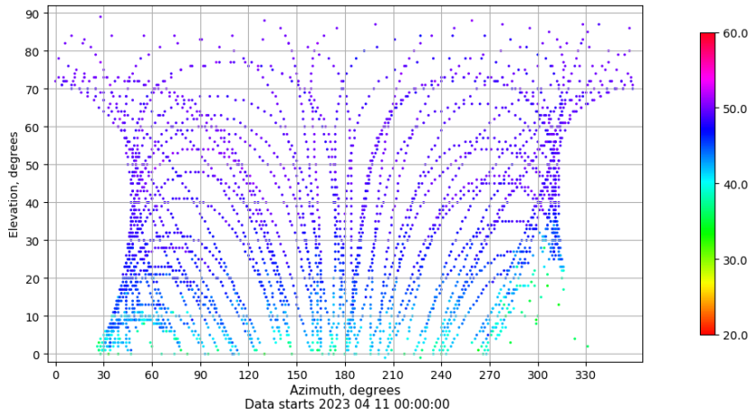
Azimuth-elevation plot for station YEB1. Signal to Noise S1C Data file YEB100ESP_R_2023101.xtr
