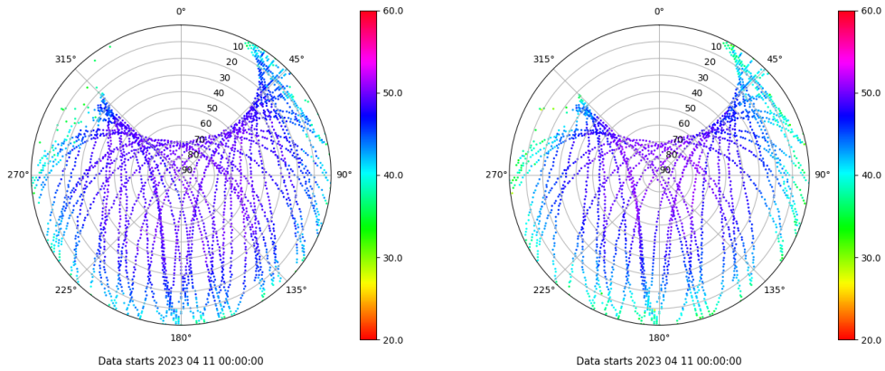
Skyplot for station YEB1. Signal to Noise S1C Data file YEB100ESP_R_2023101.xtr Skyplot for station YEB1. Signal to Noise S2S Data file YEB100ESP_R_2023101.xtr
