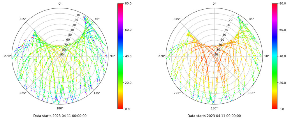
Skyplot for station YEB1. Parameter M1C Data file YEB100ESP_R_2023101.xtr Skyplot for station YEB1. Parameter M2S Data file YEB100ESP_R_2023101.xtr
