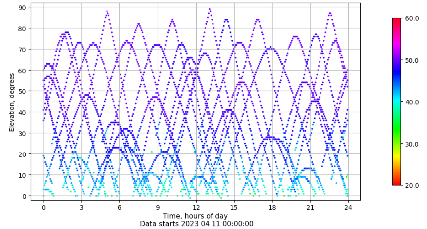
Time-elevation plot for station YEB1. Signal to Noise S1C Data file YEB100ESP_R_2023101.xtr
