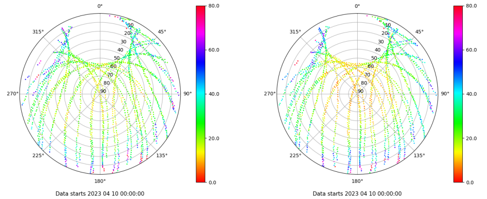
Skyplot for station YEB1. Parameter M1C Data file YEB100ESP_R_2023100.xtr Skyplot for station YEB1. Parameter M2P Data file YEB100ESP_R_2023100.xtr
