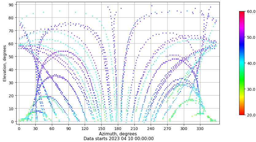
Azimuth-elevation plot for station YEB1. Signal to Noise S1C Data file YEB100ESP_R_2023100.xtr
