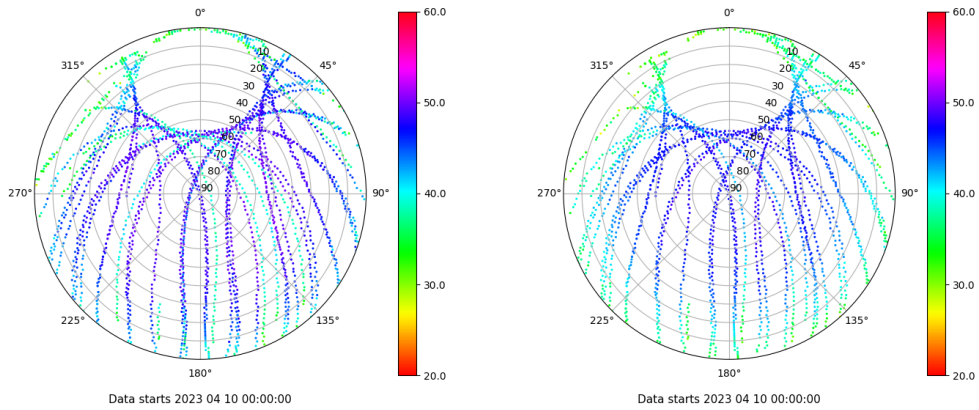
Skyplot for station YEB1. Signal to Noise S1C Data file YEB100ESP_R_2023100.xtr Skyplot for station YEB1. Signal to Noise S2P Data file YEB100ESP_R_2023100.xtr
