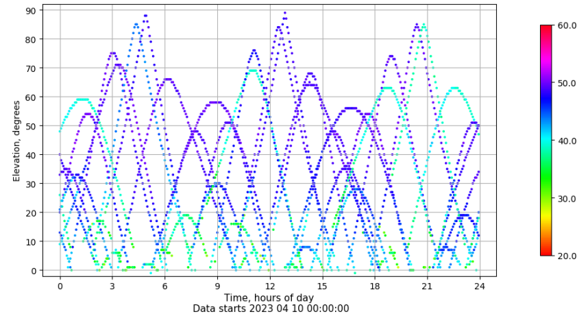
Time-elevation plot for station YEB1. Signal to Noise S1C Data file YEB100ESP_R_2023100.xtr
