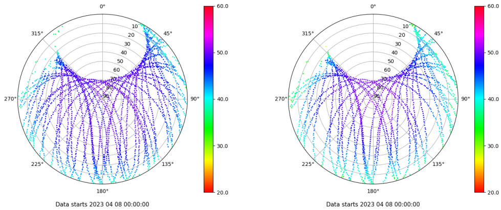
Skyplot for station YEB1. Signal to Noise S1C Data file YEB100ESP_R_2023098.xtr Skyplot for station YEB1. Signal to Noise S2S Data file YEB100ESP_R_2023098.xtr
