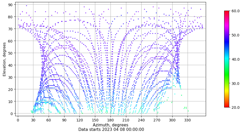
Azimuth-elevation plot for station YEB1. Signal to Noise S1C Data file YEB100ESP_R_2023098.xtr
