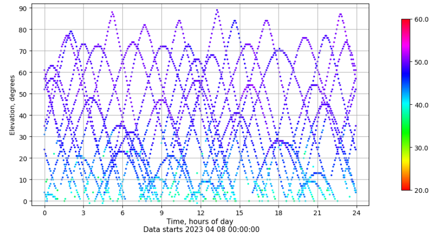
Time-elevation plot for station YEB1. Signal to Noise S1C Data file YEB100ESP_R_2023098.xtr
