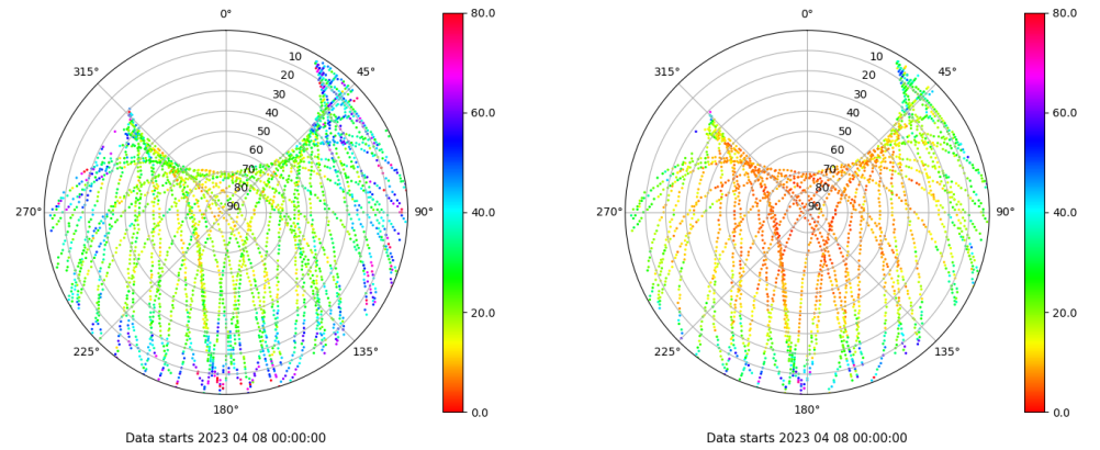
Skyplot for station YEB1. Parameter M1C Data file YEB100ESP_R_2023098.xtr Skyplot for station YEB1. Parameter M2S Data file YEB100ESP_R_2023098.xtr
