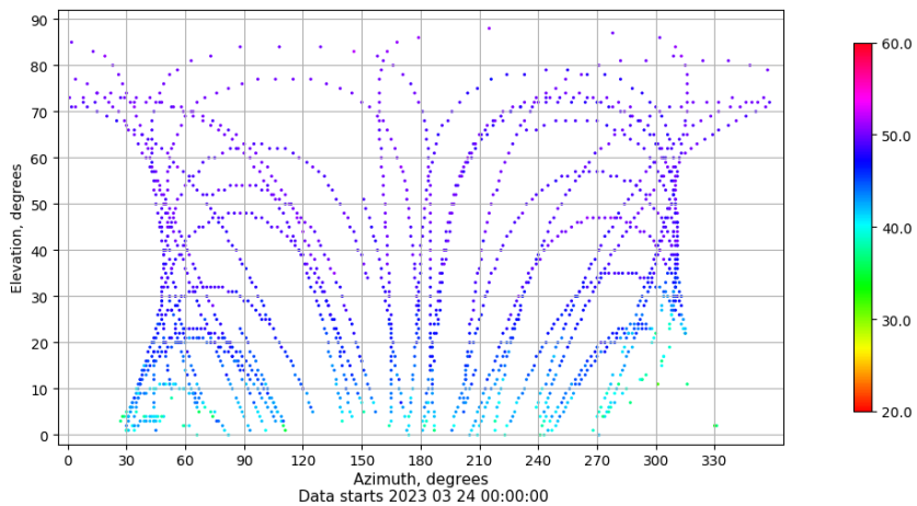
Azimuth-elevation plot for station YEB1. Signal to Noise S1C Data file YEB100ESP_R_2023083.xtr
