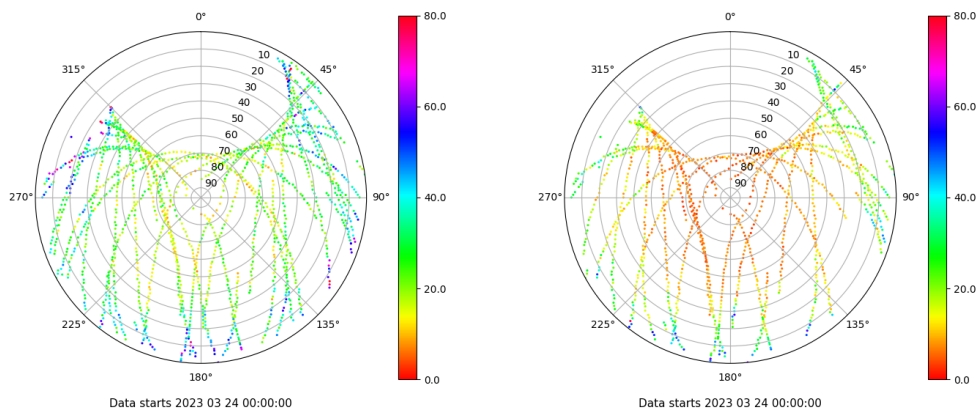
Skyplot for station YEB1. Parameter M1C Data file YEB100ESP_R_2023083.xtr Skyplot for station YEB1. Parameter M2S Data file YEB100ESP_R_2023083.xtr
