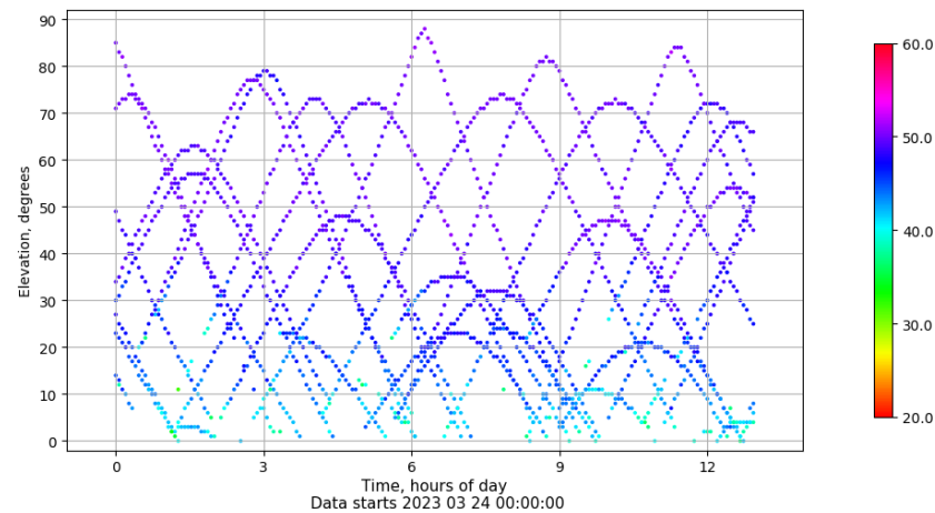
Time-elevation plot for station YEB1. Signal to Noise S1C Data file YEB100ESP_R_2023083.xtr
