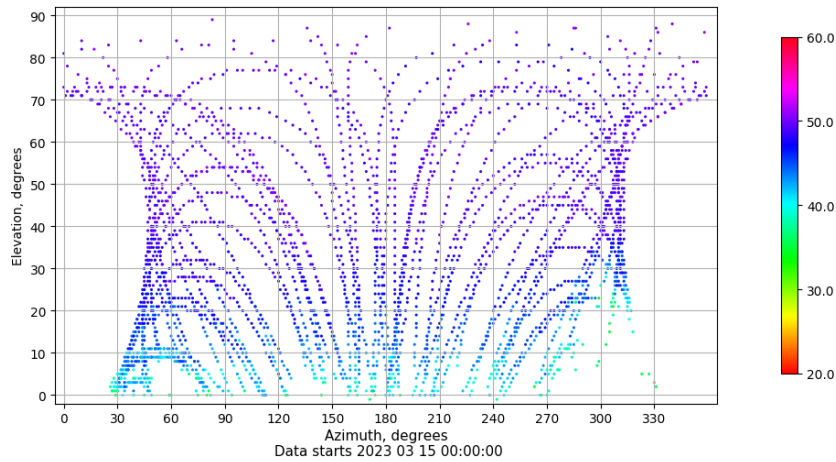
Azimuth-elevation plot for station YEB1. Signal to Noise S1C Data file YEB100ESP_R_2023074.xtr
