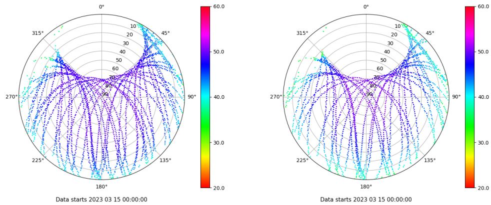
Skyplot for station YEB1. Signal to Noise S1C Data file YEB100ESP_R_2023074.xtr Skyplot for station YEB1. Signal to Noise S2S Data file YEB100ESP_R_2023074.xtr
