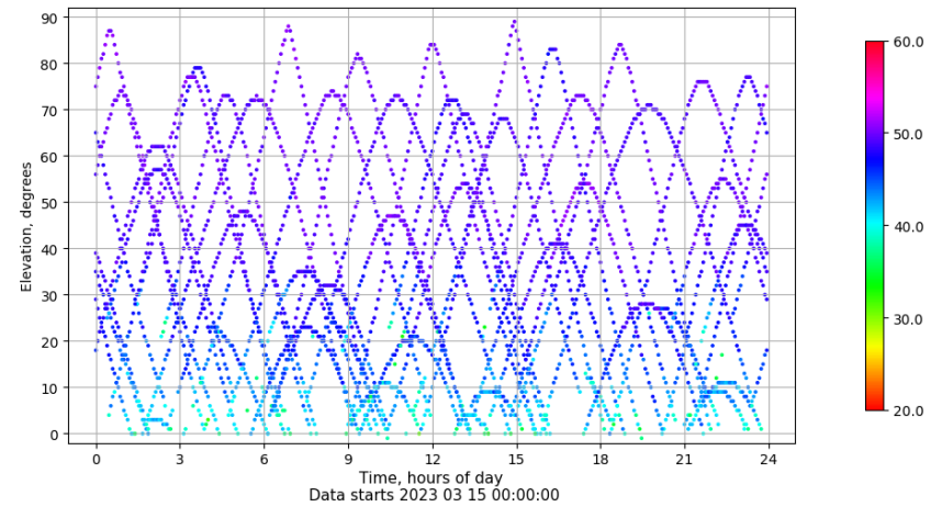
Time-elevation plot for station YEB1. Signal to Noise S1C Data file YEB100ESP_R_2023074.xtr
