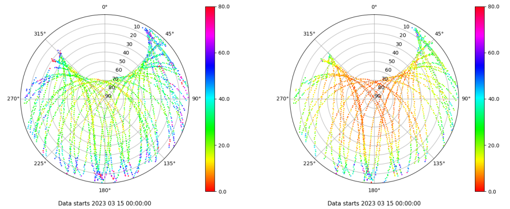
Skyplot for station YEB1. Parameter M1C Data file YEB100ESP_R_2023074.xtr Skyplot for station YEB1. Parameter M2S Data file YEB100ESP_R_2023074.xtr
