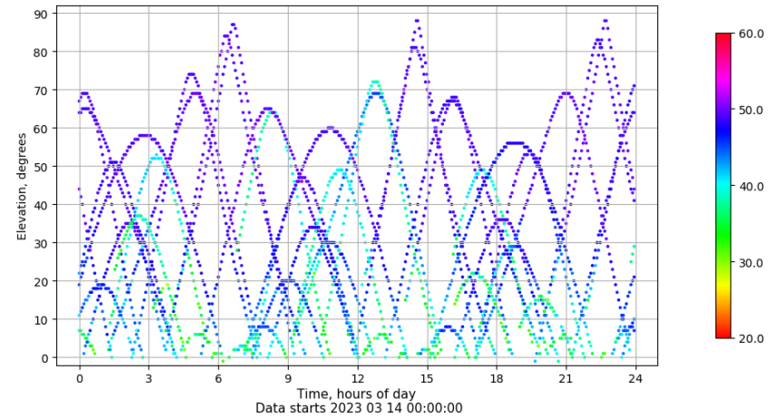
Time-elevation plot for station YEB1. Signal to Noise S1C Data file YEB100ESP_R_2023073.xtr
