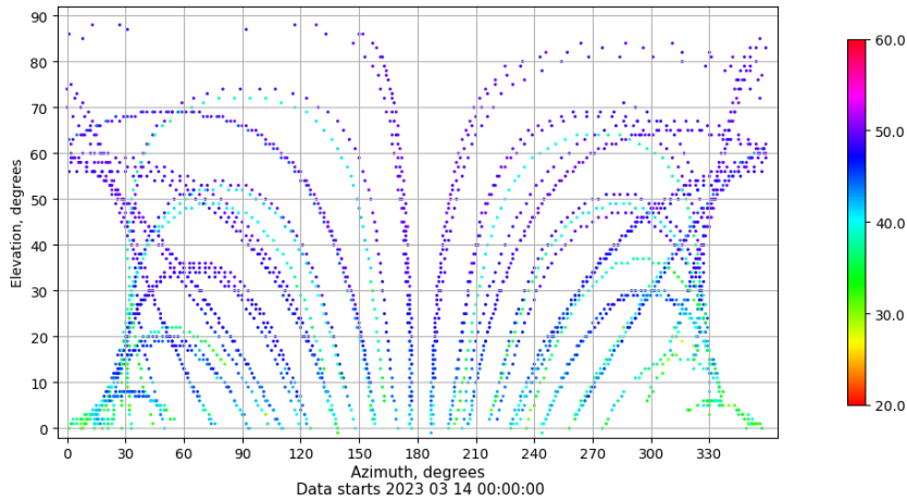
Azimuth-elevation plot for station YEB1. Signal to Noise S1C Data file YEB100ESP_R_2023073.xtr
