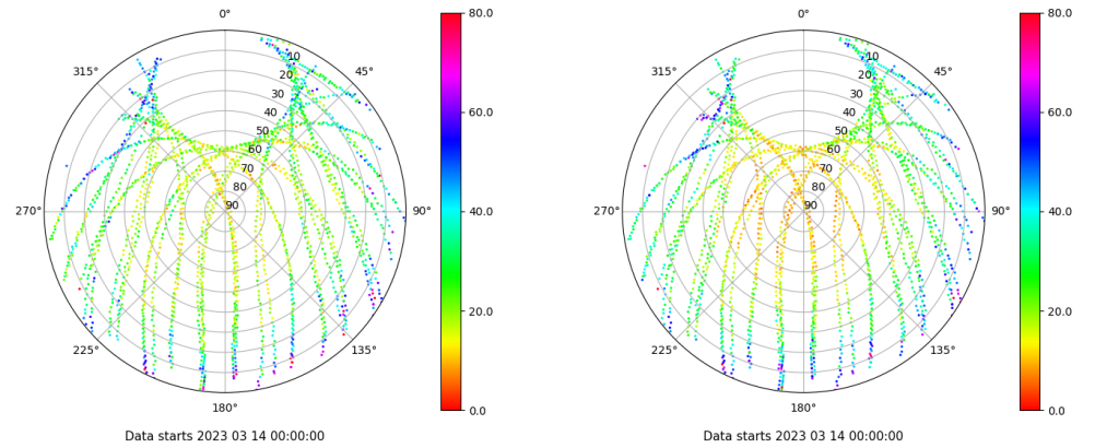
Skyplot for station YEB1. Parameter M1C Data file YEB100ESP_R_2023073.xtr Skyplot for station YEB1. Parameter M2P Data file YEB100ESP_R_2023073.xtr
