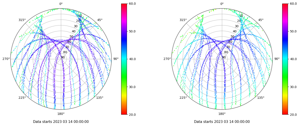
Skyplot for station YEB1. Signal to Noise S1C Data file YEB100ESP_R_2023073.xtr Skyplot for station YEB1. Signal to Noise S2P Data file YEB100ESP_R_2023073.xtr
