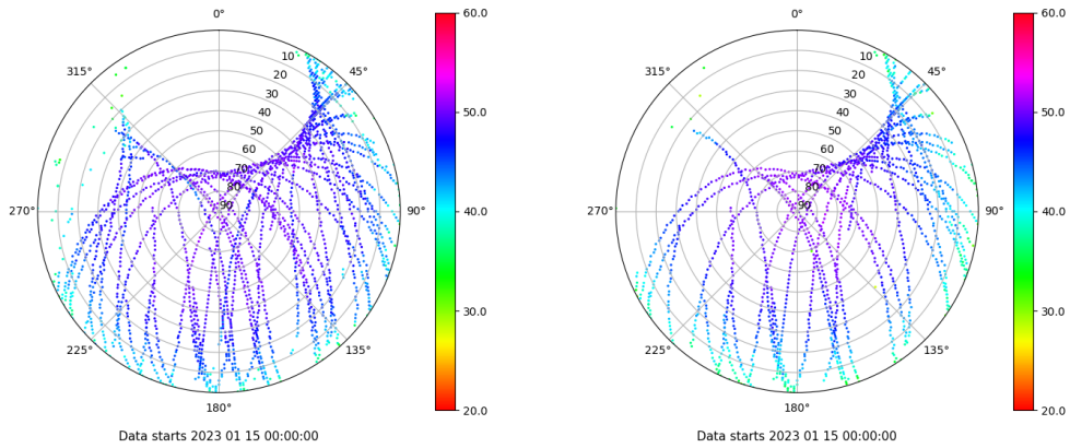
Skyplot for station YEB1. Signal to Noise S1C Data file YEB100ESP_R_2023015.xtr Skyplot for station YEB1. Signal to Noise S2S Data file YEB100ESP_R_2023015.xtr
