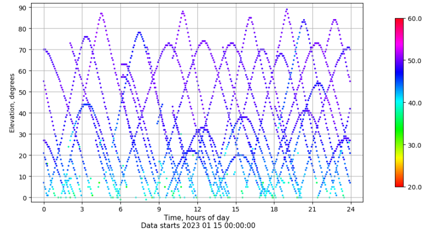
Time-elevation plot for station YEB1. Signal to Noise S1C Data file YEB100ESP_R_2023015.xtr
