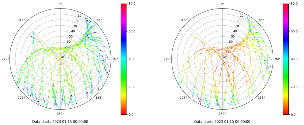
Skyplot for station YEB1. Parameter M1C Data file YEB100ESP_R_2023015.xtr Skyplot for station YEB1. Parameter M2S Data file YEB100ESP_R_2023015.xtr
