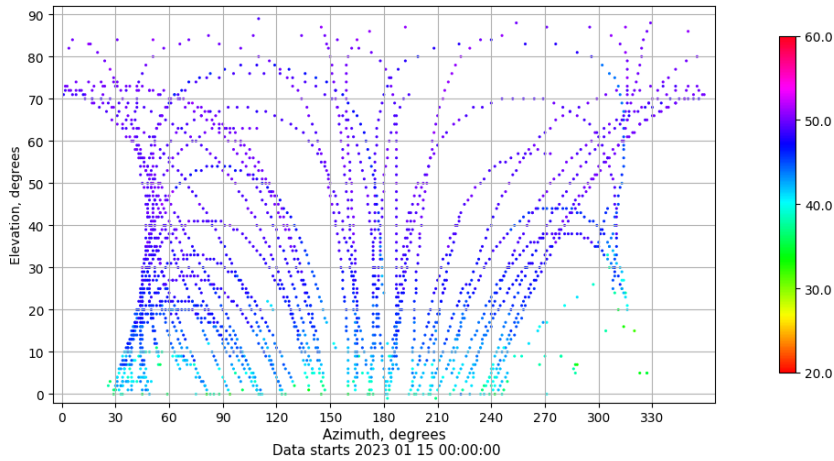
Azimuth-elevation plot for station YEB1. Signal to Noise S1C Data file YEB100ESP_R_2023015.xtr
