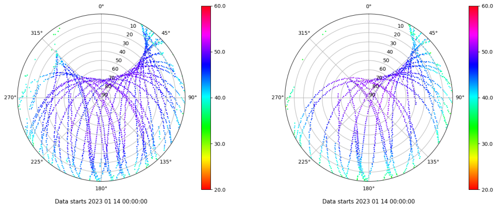
Skyplot for station YEB1. Signal to Noise S1C Data file YEB100ESP_R_2023014.xtr Skyplot for station YEB1. Signal to Noise S2S Data file YEB100ESP_R_2023014.xtr
