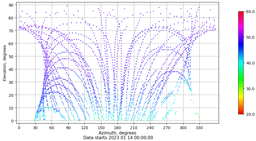
Azimuth-elevation plot for station YEB1. Signal to Noise S1C Data file YEB100ESP_R_2023014.xtr
