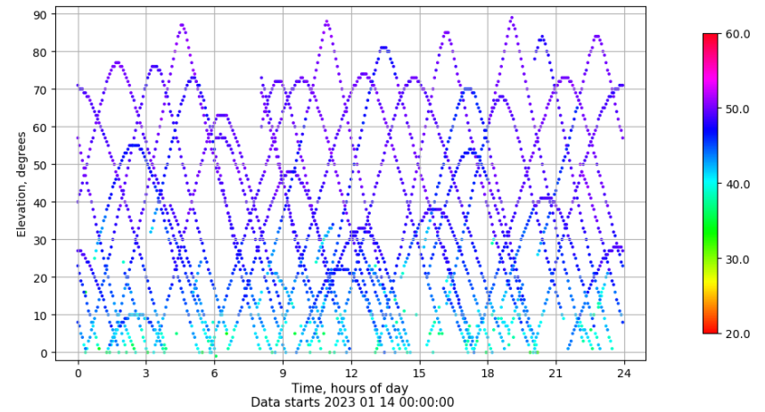
Time-elevation plot for station YEB1. Signal to Noise S1C Data file YEB100ESP_R_2023014.xtr
