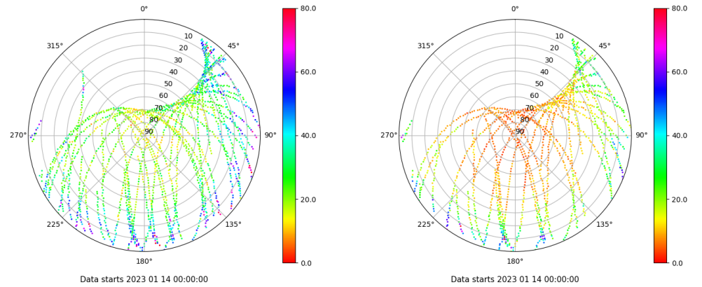
Skyplot for station YEB1. Parameter M1C Data file YEB100ESP_R_2023014.xtr Skyplot for station YEB1. Parameter M2S Data file YEB100ESP_R_2023014.xtr
