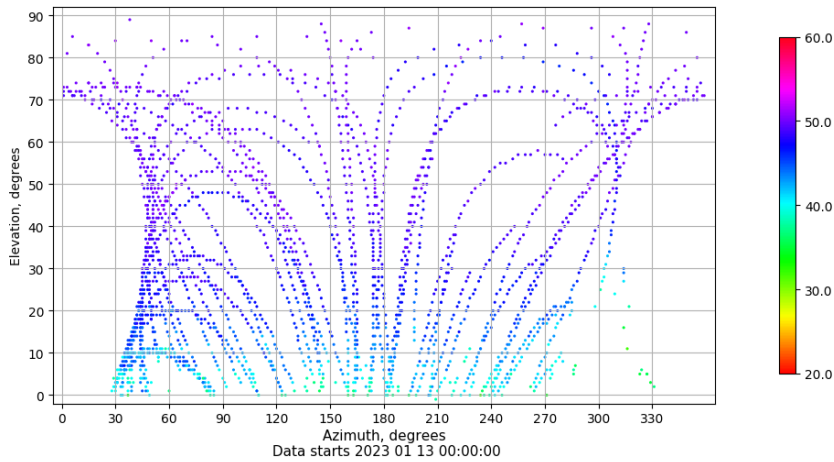
Azimuth-elevation plot for station YEB1. Signal to Noise S1C Data file YEB100ESP_R_2023013.xtr
