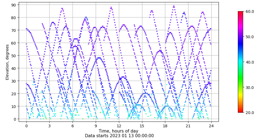
Time-elevation plot for station YEB1. Signal to Noise S1C Data file YEB100ESP_R_2023013.xtr
