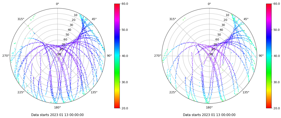
Skyplot for station YEB1. Signal to Noise S1C Data file YEB100ESP_R_2023013.xtr Skyplot for station YEB1. Signal to Noise S2S Data file YEB100ESP_R_2023013.xtr
