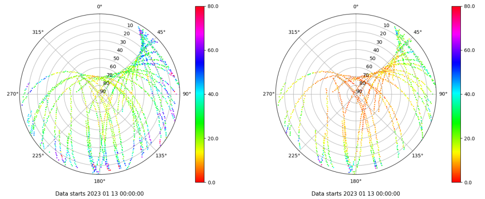
Skyplot for station YEB1. Parameter M1C Data file YEB100ESP_R_2023013.xtr Skyplot for station YEB1. Parameter M2S Data file YEB100ESP_R_2023013.xtr
