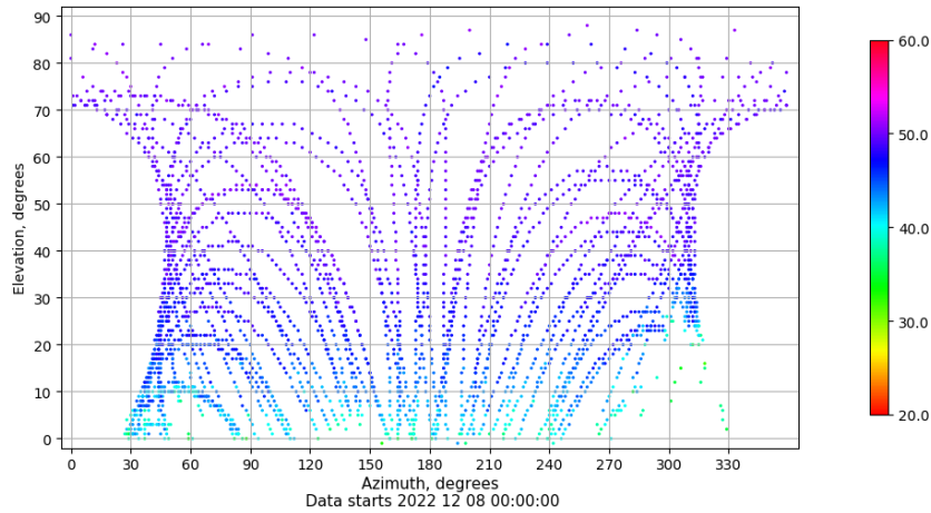
Azimuth-elevation plot for station YEB1. Signal to Noise S1C Data file YEB100ESP_R_2022342.xtr
