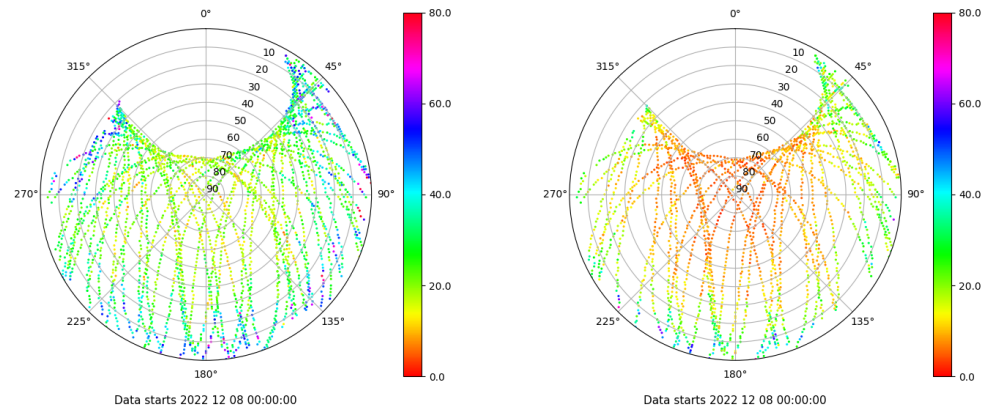
Skyplot for station YEB1. Parameter M1C Data file YEB100ESP_R_2022342.xtr Skyplot for station YEB1. Parameter M2S Data file YEB100ESP_R_2022342.xtr
