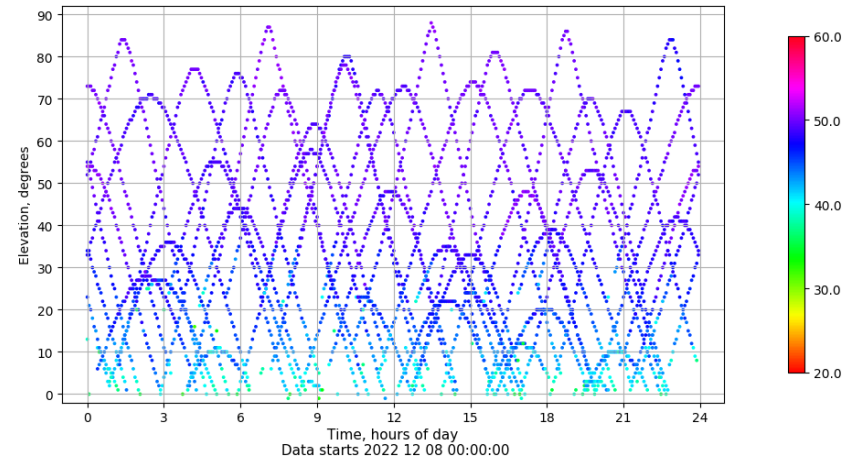
Time-elevation plot for station YEB1. Signal to Noise S1C Data file YEB100ESP_R_2022342.xtr
