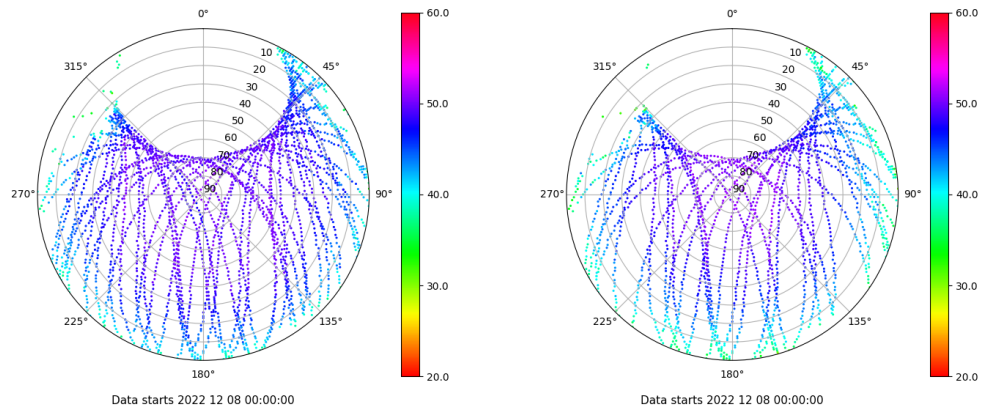
Skyplot for station YEB1. Signal to Noise S1C Data file YEB100ESP_R_2022342.xtr Skyplot for station YEB1. Signal to Noise S2S Data file YEB100ESP_R_2022342.xtr
