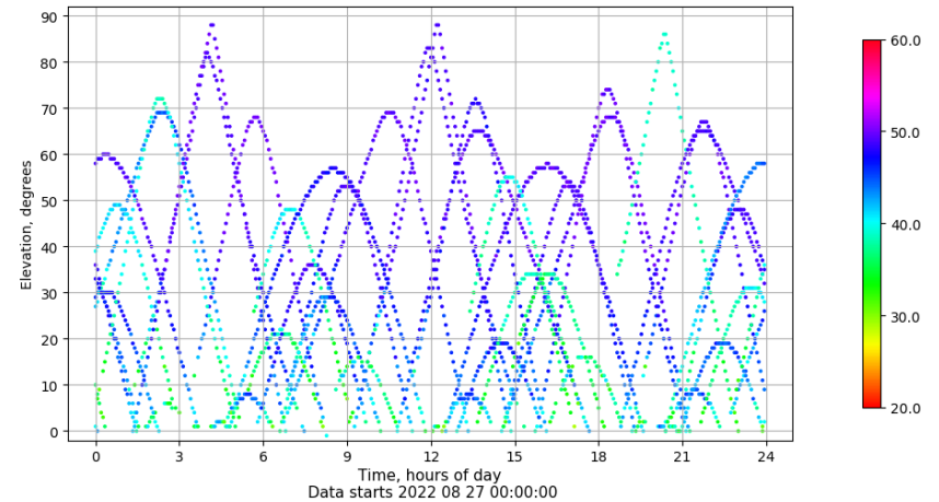
Time-elevation plot for station YEB1. Signal to Noise S1C Data file YEB100ESP_R_2022239.xtr
