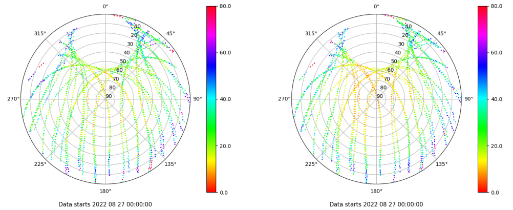
Skyplot for station YEB1. Parameter M1C Data file YEB100ESP_R_2022239.xtr Skyplot for station YEB1. Parameter M2P Data file YEB100ESP_R_2022239.xtr
