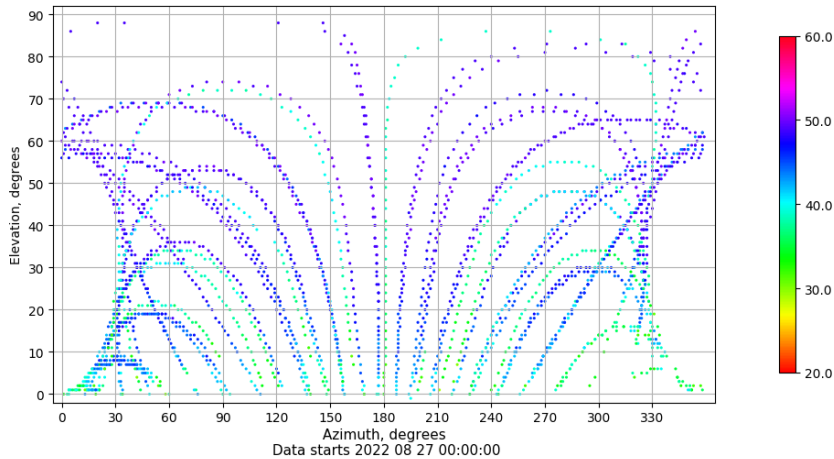
Azimuth-elevation plot for station YEB1. Signal to Noise S1C Data file YEB100ESP_R_2022239.xtr
